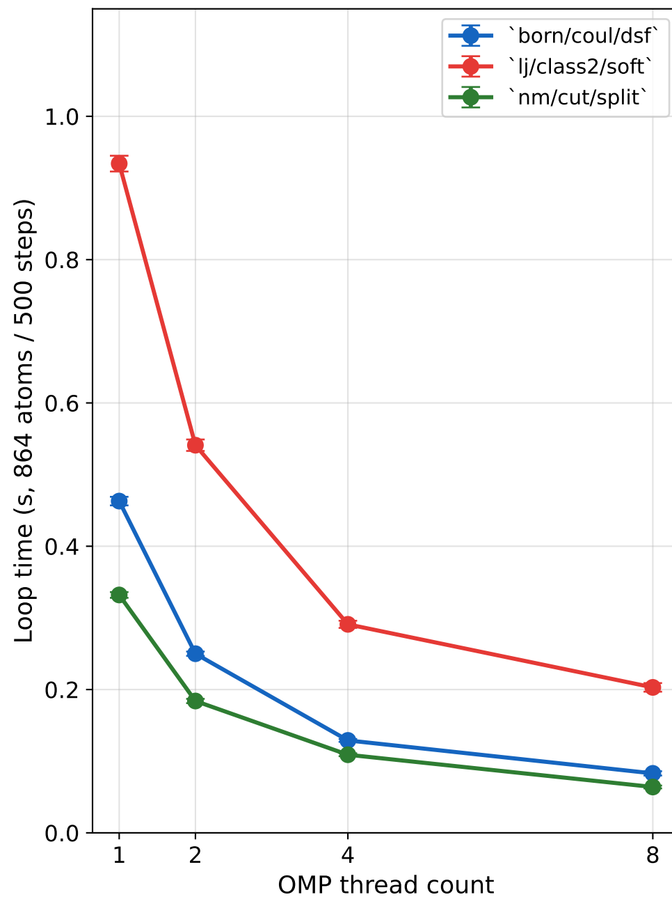
(a) Loop time vs. thread count (N=3 runs, error bars \pm 1\sigma )
