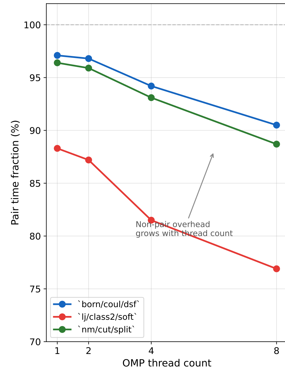
(c) Pair-time fraction vs. thread count (Amdahl limit from non-pair overhead)
