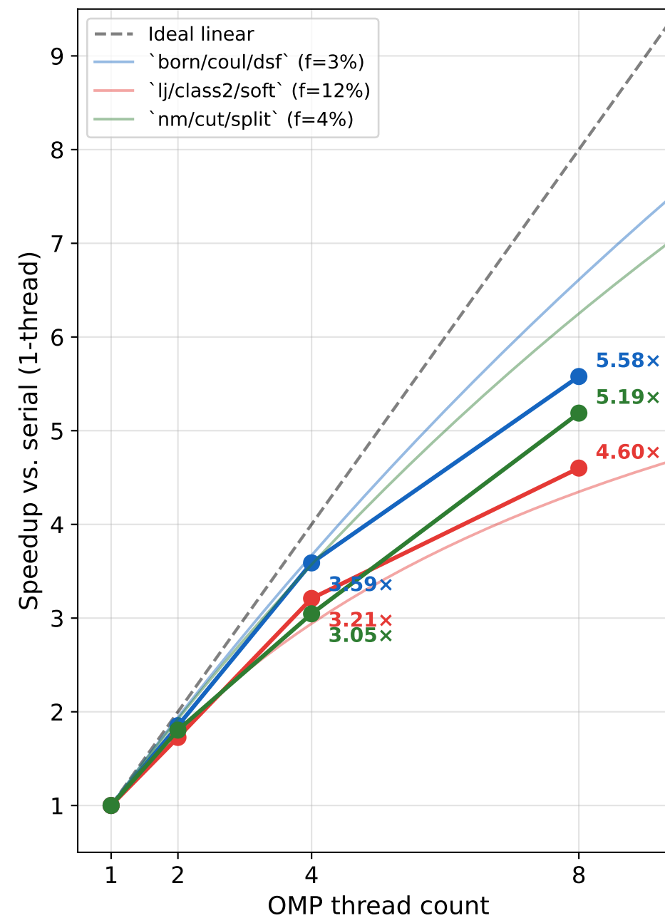
(b) Speedup and Amdahl's law fit (f = serial fraction)
