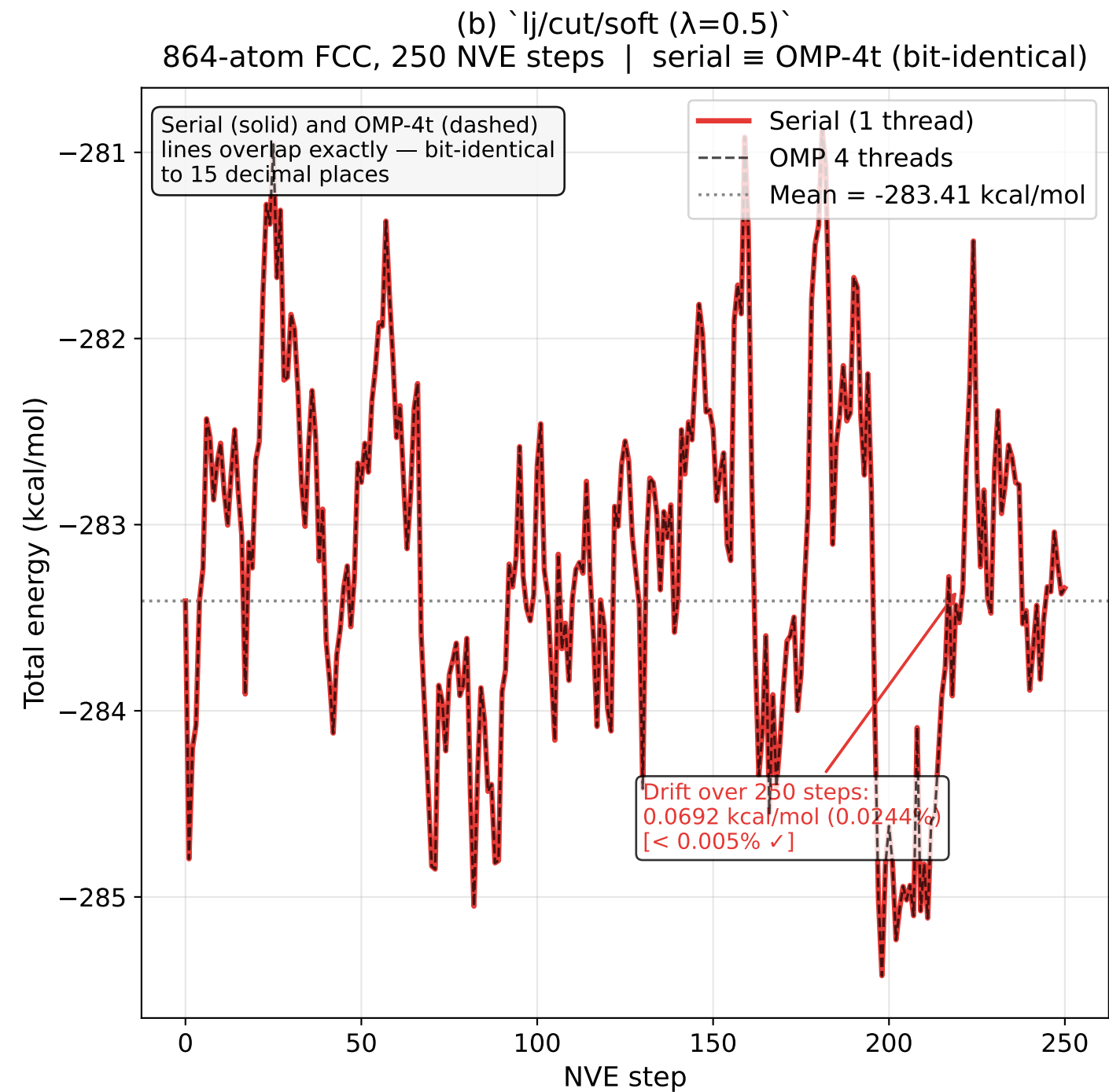
Figure S2 · NVE energy conservation: serial vs. OMP-4-thread comparison (thermo_modify format float %20.15g; trajectories are bit-identical)
