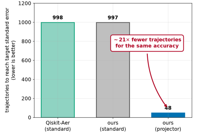
FIGURE 6. Head-to-head against Qiskit-Aer. Bar height is the number of trajectories (equivalently shots) needed to reach the target standard error SE \leq 10^{-2} on the observable \frac{1}{n} \sum_i X_i ; lower is better. Conditions: n = 10 , strong noise \gamma t = 1.5 , exact mean e^{-2\gamma t} = 0.0498 , all three methods reproduce it (Table 4). Left (green): Qiskit-Aer’s production batched_shots_gpu standard unraveling, 998. Middle (black): our engine’s standard unraveling, 997—statistically indistinguishable from Aer, which certifies that our engine is a faithful, apples-to-apples baseline and that the improvement is due to the unraveling, not the implementation. Right (blue): our projector unraveling, 48—a \sim 21\times reduction (red arrow) at identical accuracy. Wall-clock is discussed separately (Sec. VII): the saving is in trajectory count , an engine-independent statistical quantity that a compiled implementation would convert into proportional wall-clock.
