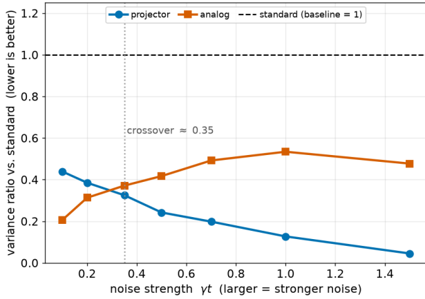
FIGURE 3. Regime map of unraveling efficiency. The x -axis is the accumulated noise strength \gamma t (larger = stronger noise); the y -axis is the per-trajectory variance of the estimator relative to the standard unraveling , so lower is better and the black dashed line at 1 is the standard baseline. Blue circles are projector, orange squares are analog (single dephasing channel, n = 12 , N = 2 \times 10^3 ). Both curves lie entirely below 1, i.e. both variance-reduced unravelings beat standard at every noise level. The projector ratio falls monotonically to 0.045 at \gamma t = 1.5 (a \sim 22\times variance reduction), while analog is lowest at weak noise; the two curves cross near \gamma t \approx 0.35 (grey dotted). Practical reading: use analog to the left of the crossover and projector to the right. Because deeper or larger noisy circuits accumulate more \gamma t , they fall into the projector-favorable (right) region.
