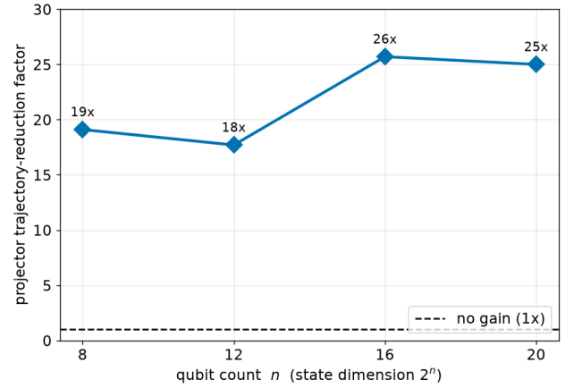
FIGURE 4. Scaling of the trajectory-reduction factor. The x -axis is the qubit count n (state dimension 2^n , i.e. 256 to \sim 10^6 amplitudes); the y -axis is how many times fewer trajectories the projector unraveling needs than standard to reach the same target standard error ( SE \leq 10^{-2} , strong noise \gamma t = 1.5 ). Each blue marker is a measured ratio (Table 3); the black dashed line at 1 marks “no advantage”. The factor stays in the 19\text{--}26\times band with no downward trend across n = 8\text{--}20 , so the benefit is a statistical property of the unraveling rather than a small-system artifact. Statevector memory is only 16.8 MB at n = 20 , four orders of magnitude below the 8 GB budget, indicating the method is compute-bound here and that the same advantage is expected to persist to the \sim 30 -qubit regime reachable on larger-memory GPUs.
