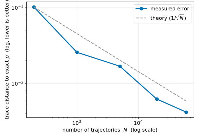
FIGURE 2. Correctness of the GPU trajectory engine. We reconstruct the density matrix \rho = \frac{1}{N} \sum_i |\psi^{(i)}\rangle\langle\psi^{(i)}| from N standard-unraveling trajectories and plot its trace distance to Qiskit-Aer’s exact density_matrix result, on log-log axes; the x -axis is the number of trajectories N ( 2 \times 10^2 to 6 \times 10^4 ) and the y -axis is the trace distance (lower is more accurate). Blue circles are the measured error; the grey dashed line is the theoretical Monte-Carlo rate \propto 1/\sqrt{N} anchored at the first point. The measured error falls from 0.101 to 4.2 \times 10^{-3} and lies on the 1/\sqrt{N} reference throughout (the product D \cdot \sqrt{N} stays near 1.0), so the estimator is unbiased and converges at the statistically optimal rate—establishing that “fewer trajectories” (Figs. 3–6) is a genuine efficiency gain, not a loss of accuracy. System: 6-qubit circuit, depolarizing noise on single-qubit gates, reference purity \text{Tr} \rho^2 = 0.61 .
