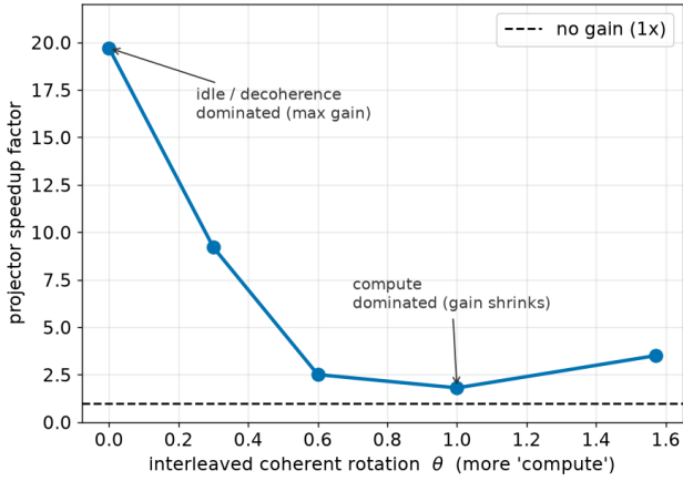
FIGURE 5. Applicability map: coherent dynamics erodes the projector advantage. The x -axis is the angle \theta of R_Y(\theta) rotations interleaved between noise windows—a proxy for how much coherent “compute” the circuit performs relative to idle decoherence; the y -axis is the projector trajectory-reduction factor ( n = 8 , \gamma t = 1.5 ). At \theta = 0 (pure idle/dephasing, the absorbing-window ideal) the speedup is largest, 19.7\times ; it falls monotonically to 1.8\times at \theta = 1.0 as R_Y (which does not commute with the measured X ) repeatedly rotates collapsed states back out of the absorbing subspace, with a partial rebound to 3.5\times at \theta = \pi/2 . Crucially the estimator mean remains unbiased at every \theta (it always tracks the exact value); only the size of the variance advantage changes. The practical message is that projector unraveling pays off most for decoherence/idle-dominated workloads (e.g. quantum-memory and long-delay circuits), which is precisely where noisy-simulation cost is otherwise highest.
