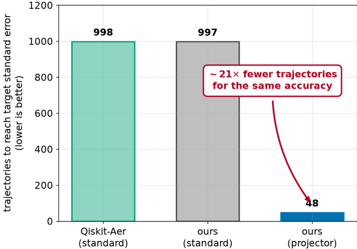
Figure 6: Head-to-head against Qiskit-Aer. Bar height is the number of trajectories (equivalently shots) needed to reach the target standard error SE \leq 10^{-2} on the observable \frac{1}{n} \sum_i X_i ; lower is better. Conditions: n = 10 , strong noise \gamma t = 1.5 , exact mean e^{-2\gamma t} = 0.0498 , all three methods reproduce it (Table 4). Left (green): Qiskit-Aer’s production batched_shots_gpu standard unraveling, 998. Middle (black): our engine’s standard unraveling, 997—statistically indistinguishable from Aer, which certifies that our engine is a faithful, apples-to-apples baseline and that the improvement is due to the unraveling, not the implementation. Right (blue): our projector unraveling, 48—a \sim 21\times reduction (red arrow) at identical accuracy. Wall-clock is discussed separately (Section 7): the saving is in trajectory count , an engine-independent statistical quantity that a compiled implementation would convert into proportional wall-clock.
