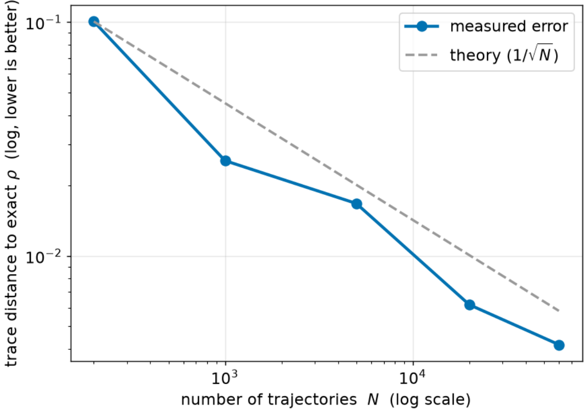
Figure 2: Correctness of the GPU trajectory engine. We reconstruct the density matrix \rho = \frac{1}{N} \sum_i |\psi^{(i)}\rangle\langle\psi^{(i)}| from N standard-unraveling trajectories and plot its trace distance to Qiskit-Aer’s exact density_matrix result, on log-log axes; the x -axis is the number of trajectories N ( 2 \times 10^2 to 6 \times 10^4 ) and the y -axis is the trace distance (lower is more accurate). Blue circles are the measured error; the grey dashed line is the theoretical Monte-Carlo rate \propto 1/\sqrt{N} anchored at the first point. The measured error falls from 0.101 to 4.2 \times 10^{-3} and lies on the 1/\sqrt{N} reference throughout (the product D \cdot \sqrt{N} stays near 1.0), so the estimator is unbiased and converges at the statistically optimal rate—establishing that “fewer trajectories” (Figs. 3–6) is a genuine efficiency gain, not a loss of accuracy. System: 6-qubit circuit, depolarizing noise on single-qubit gates, reference purity \text{Tr } \rho^2 = 0.61 .
