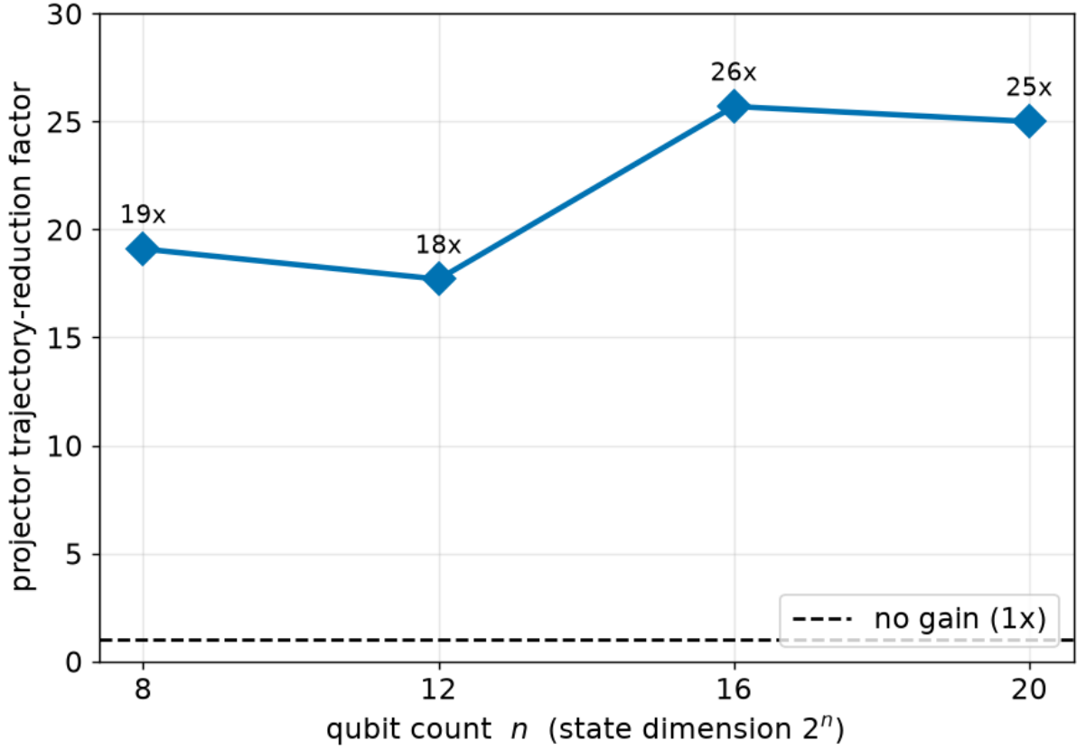
Figure 4: Scaling of the trajectory-reduction factor. The x -axis is the qubit count n (state dimension 2^n , i.e. 256 to \sim 10^6 amplitudes); the y -axis is how many times fewer trajectories the projector unraveling needs than standard to reach the same target standard error ( SE \leq 10^{-2} , strong noise \gamma t = 1.5 ). Each blue marker is a measured ratio (Table 3); the black dashed line at 1 marks “no advantage”. The factor stays in the 19–26 \times band with no downward trend across n = 8 –20, so the benefit is a statistical property of the unraveling rather than a small-system artifact. Statevector memory is only 16.8 MB at n = 20 , four orders of magnitude below the 8 GB budget, indicating the method is compute-bound here and that the same advantage is expected to persist to the \sim 30 -qubit regime reachable on larger-memory GPUs.
