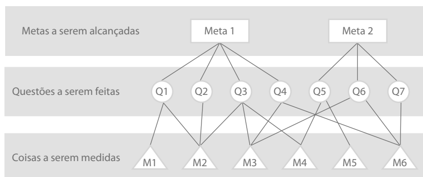
Figura 26.3 O paradigma GQM
