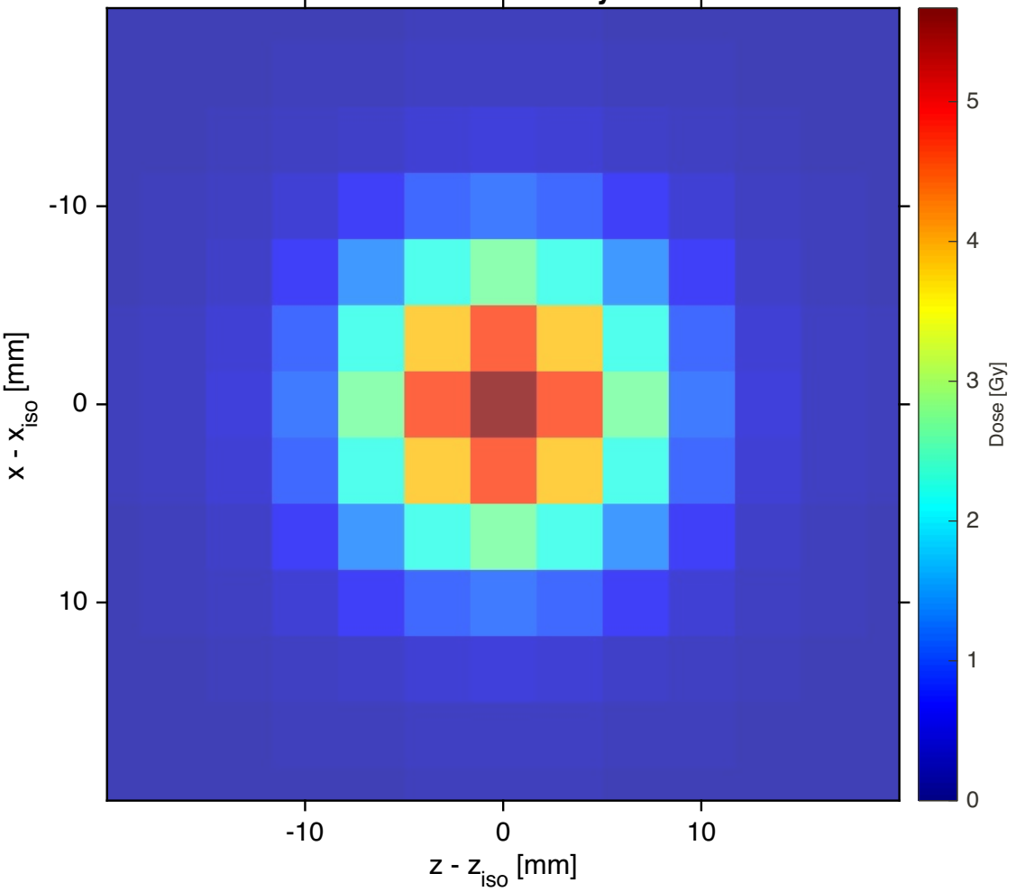
MAX 181.01 MeV: beam's-eye at 218 mm
