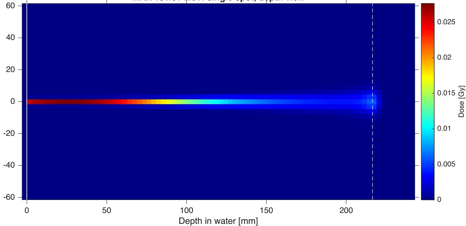
MAX 181.01 MeV: single spot, depth view
