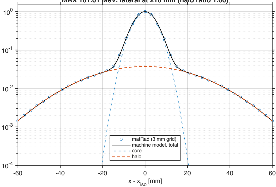
MAX 181.01 MeV: lateral at 218 mm (halo ratio 1.00)
