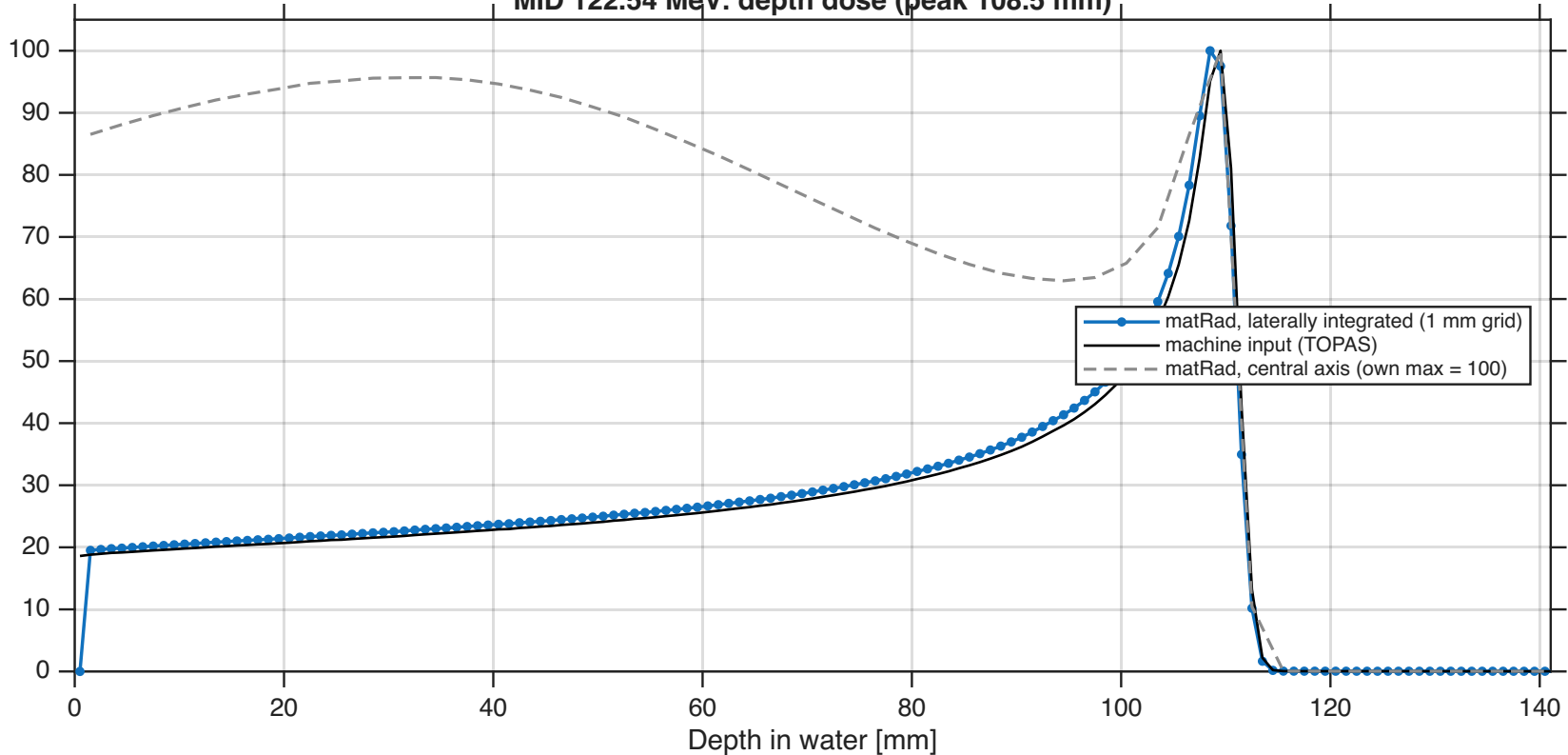
MID 122.54 MeV: depth dose (peak 108.5 mm)
