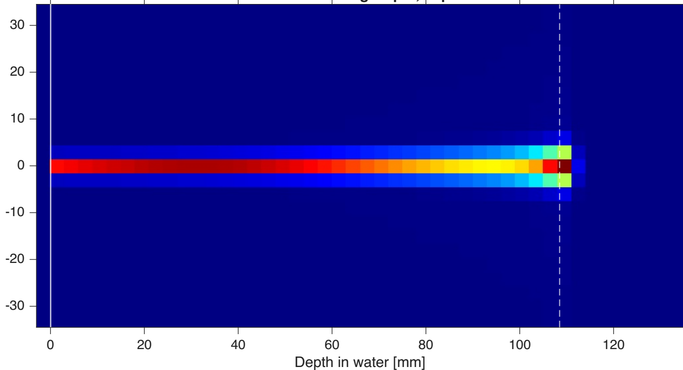
MID 122.54 MeV; single spot, depth view
