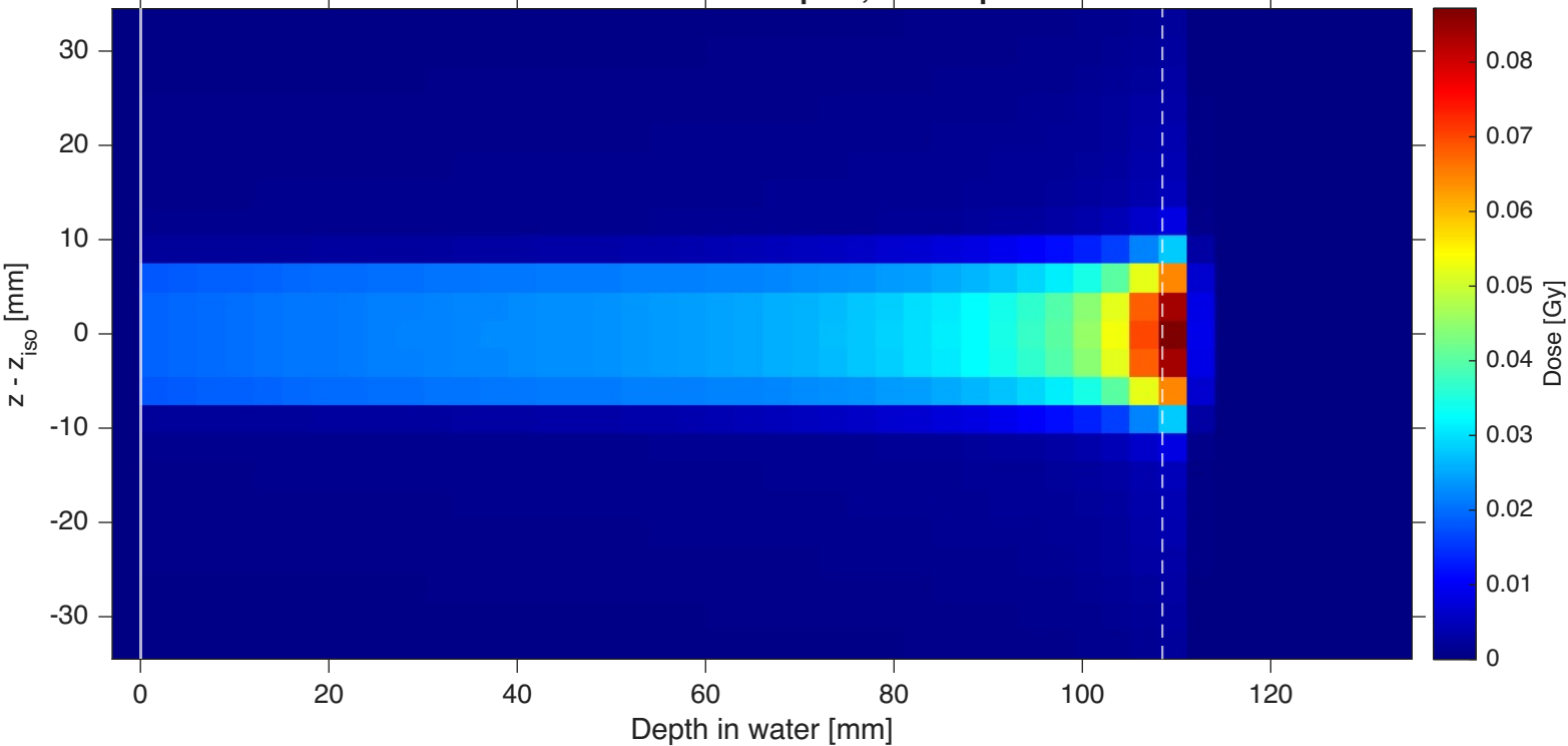
MID 122.54 MeV: 5x5 spots, 3 mm apart
