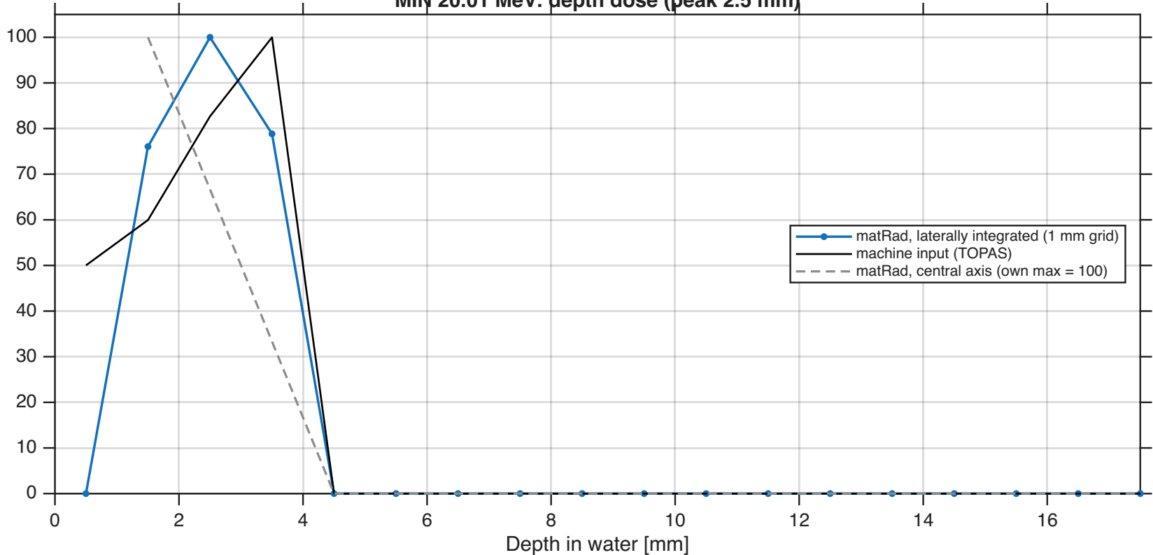
MIN 20.01 MeV: depth dose (peak 2.5 mm)
