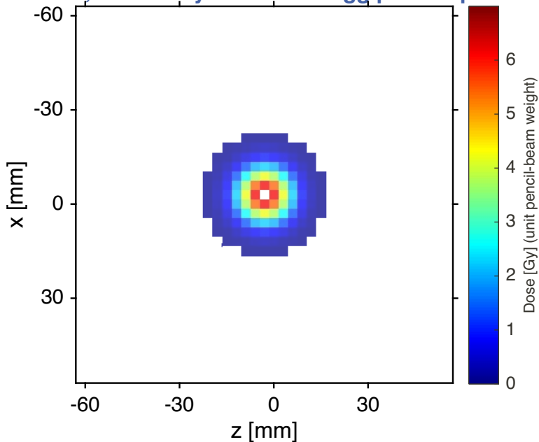
DWA_proton dose, beam's-eye view at Bragg peak depth @ 149.2 MeV
