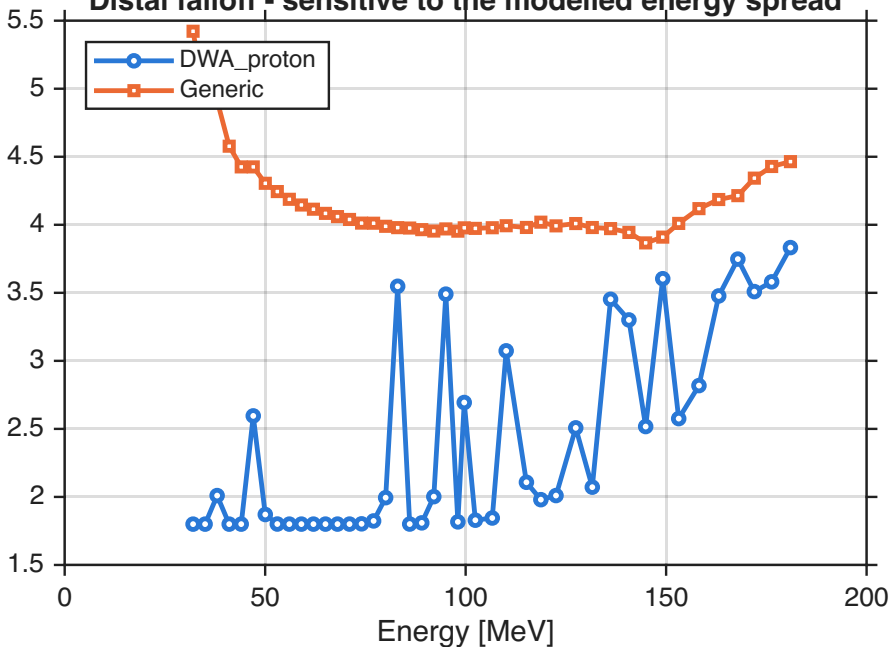
Distal falloff - sensitive to the modelled energy spread
