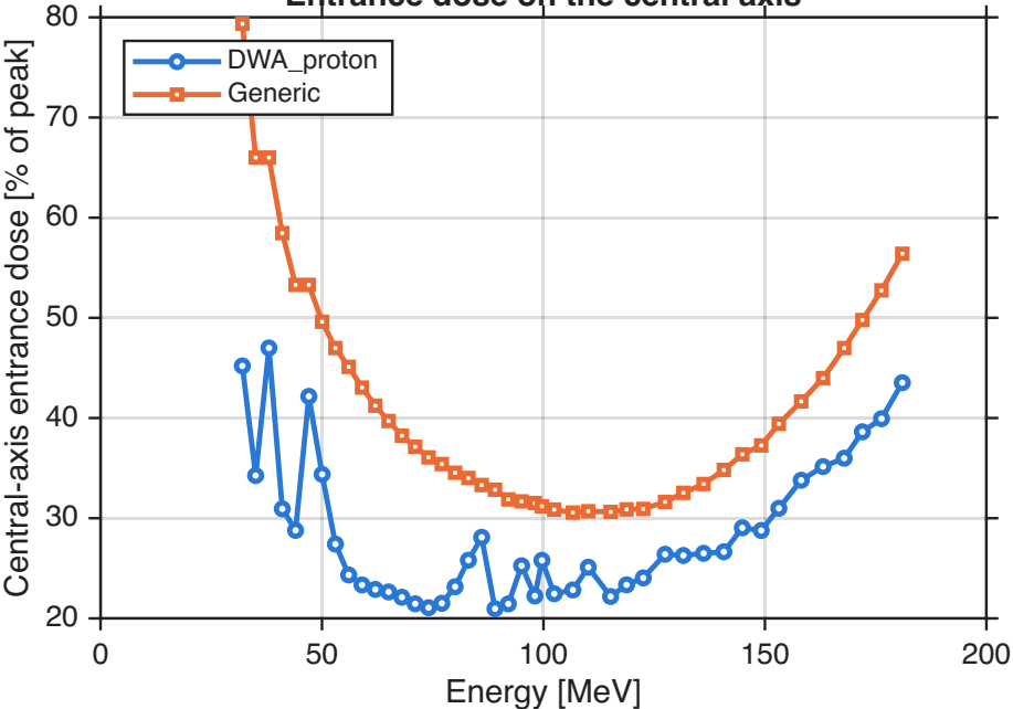
Entrance dose on the central axis
