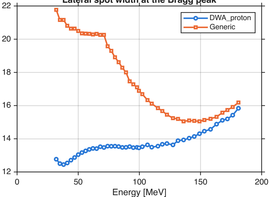
Lateral spot width at the Bragg peak
