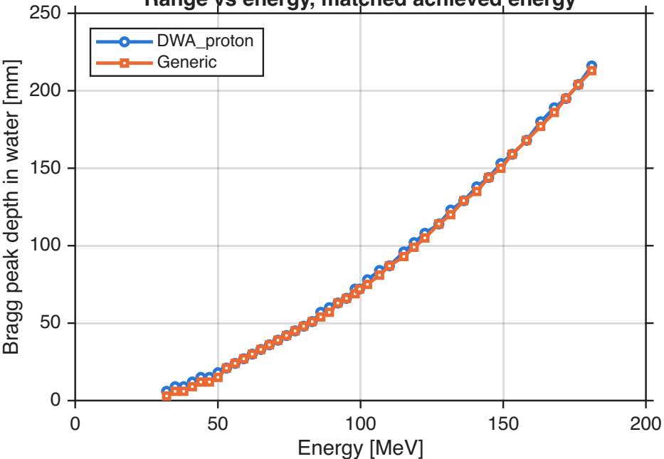
Range vs energy, matched achieved energy
