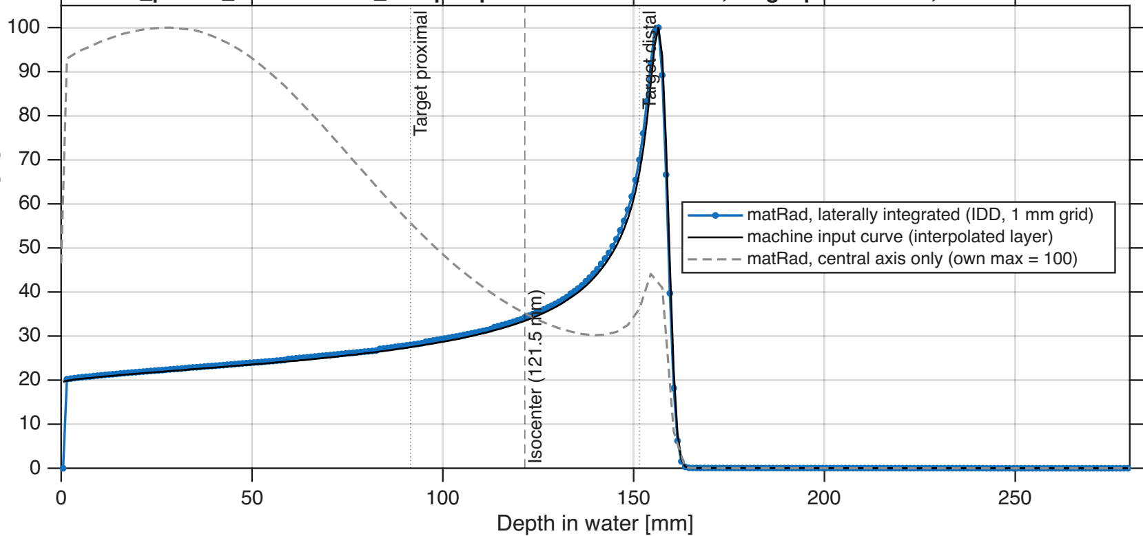
DWA_proton_doubleGauss_interp depth dose @ 150.16 MeV, single pencil beam, BOXPHANTOM
