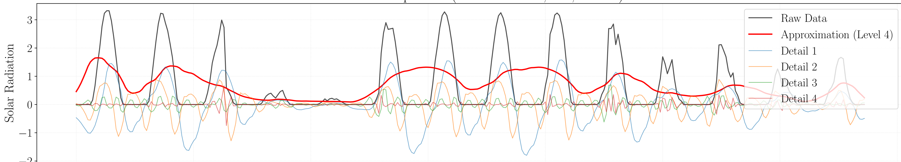
Wavelet Decomposition (Additive Model, db4, Level 4)
