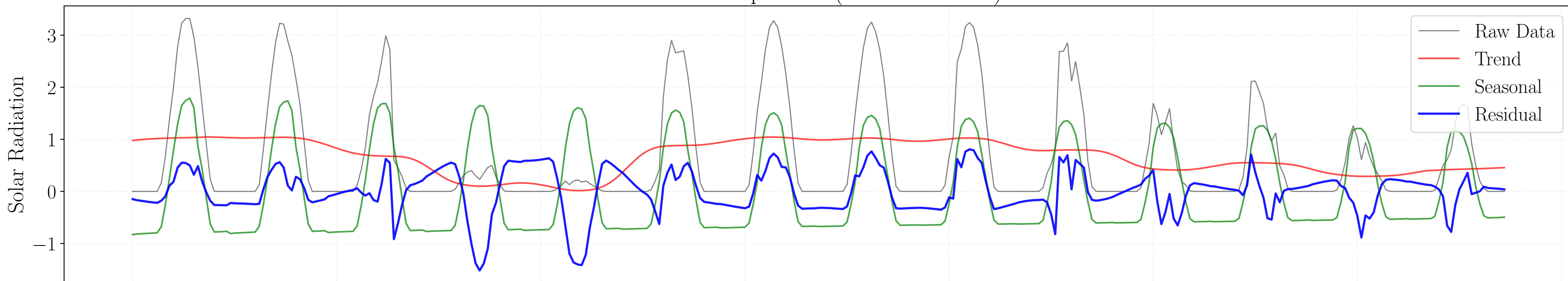
STL Decomposition (Additive Model)
