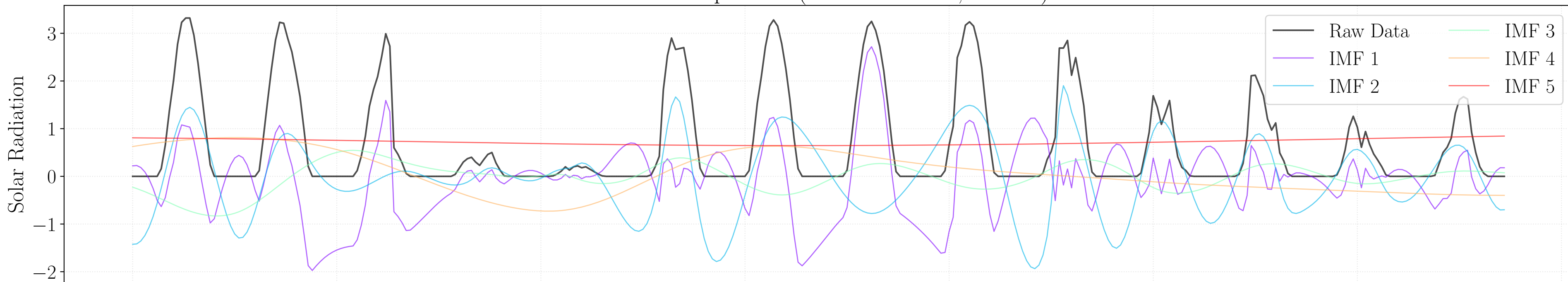
EMD Decomposition (Additive Model, 5 IMFs)
