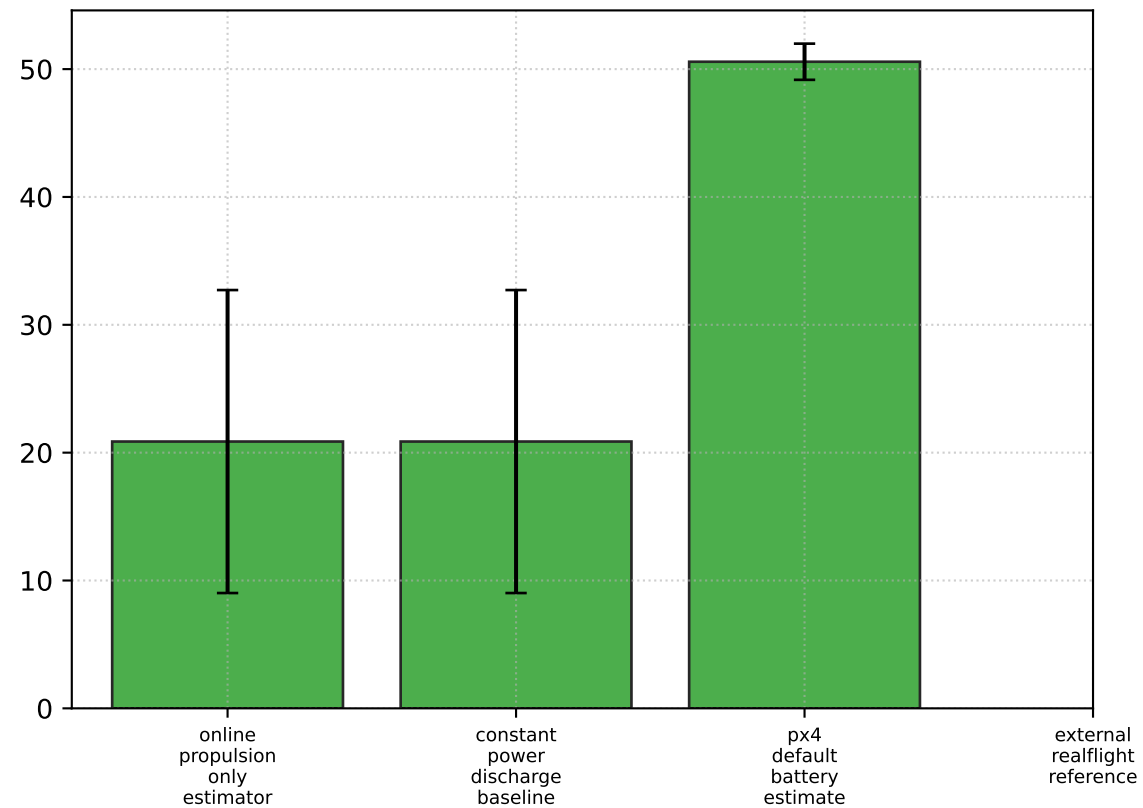
Final SOC by model (%)
