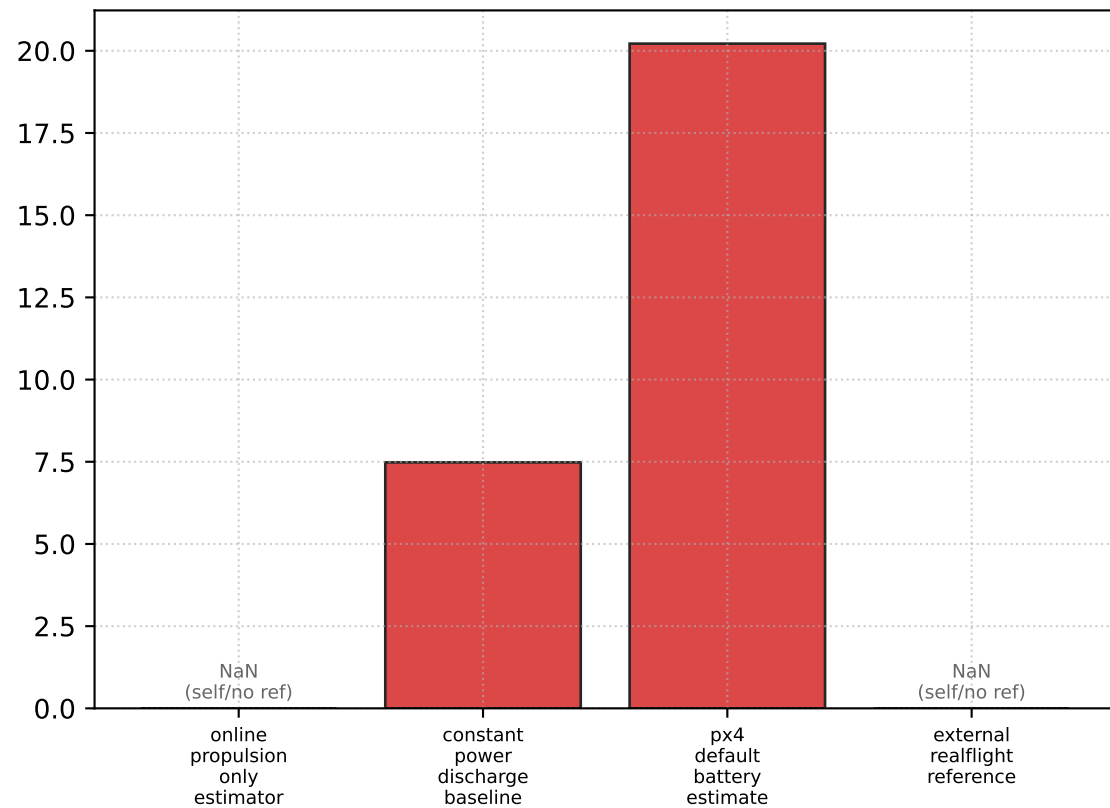
SOC RMSE vs online estimator (%)
