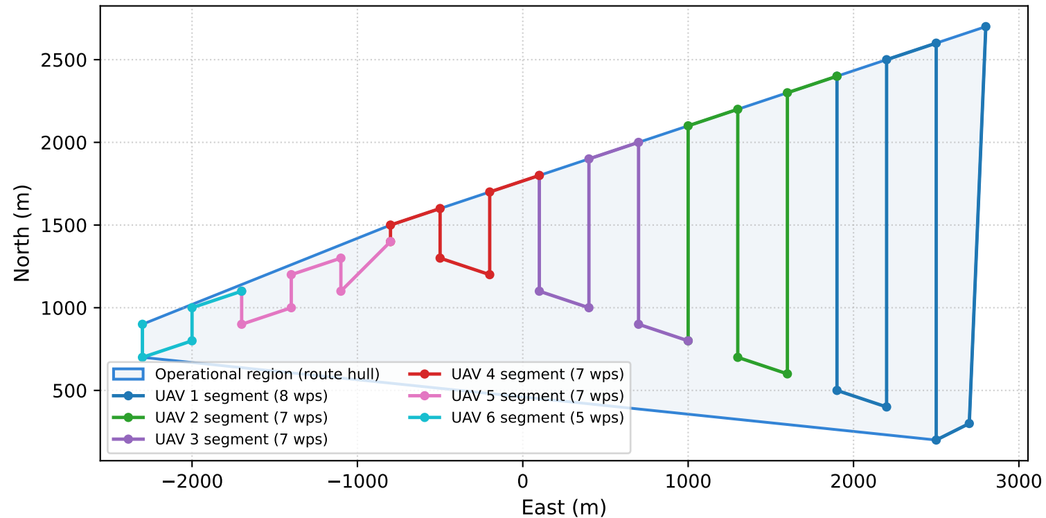
Evaluation region and partitioned coverage route (total 23.3 km, 6 UAVs)
