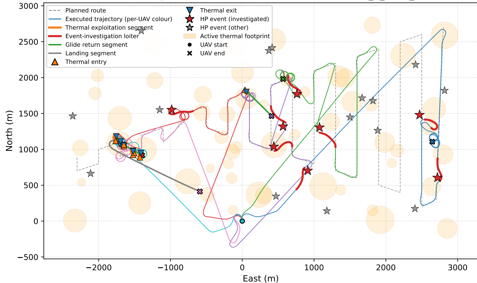
Executed trajectories vs planned route — nominal/N_6_seed_42
