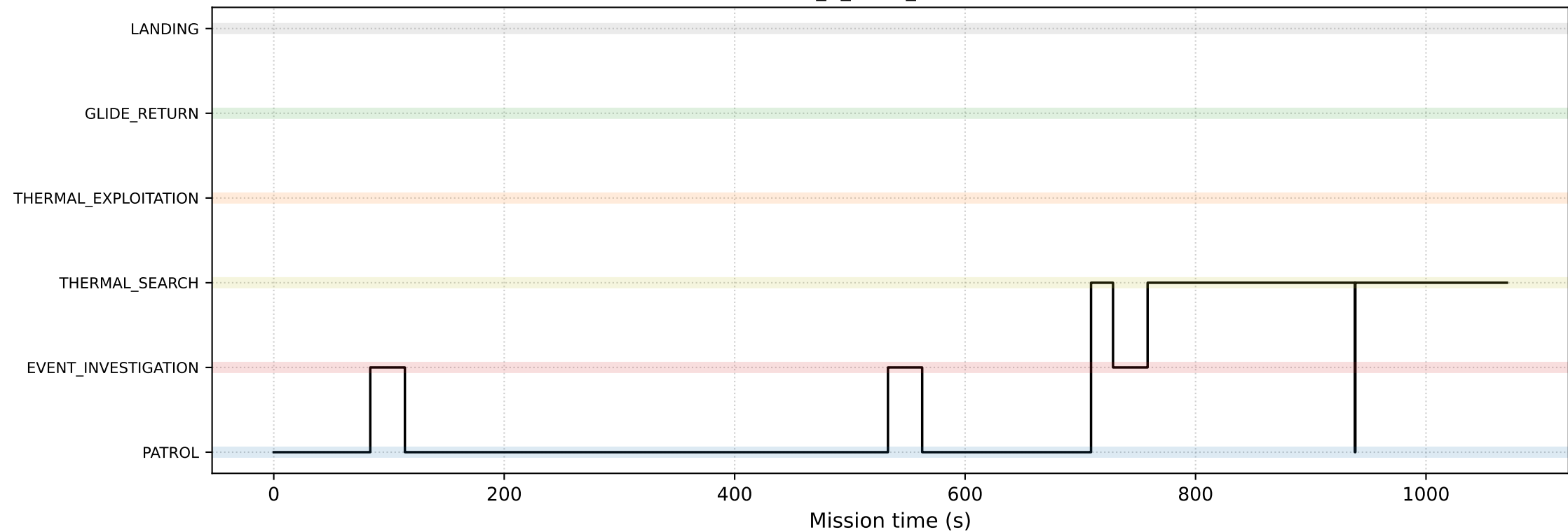
FSM transition timeline — UAV 1, nominal/N_6_seed_42 (9 transitions, stabilized: no sub-2 s chatter)
