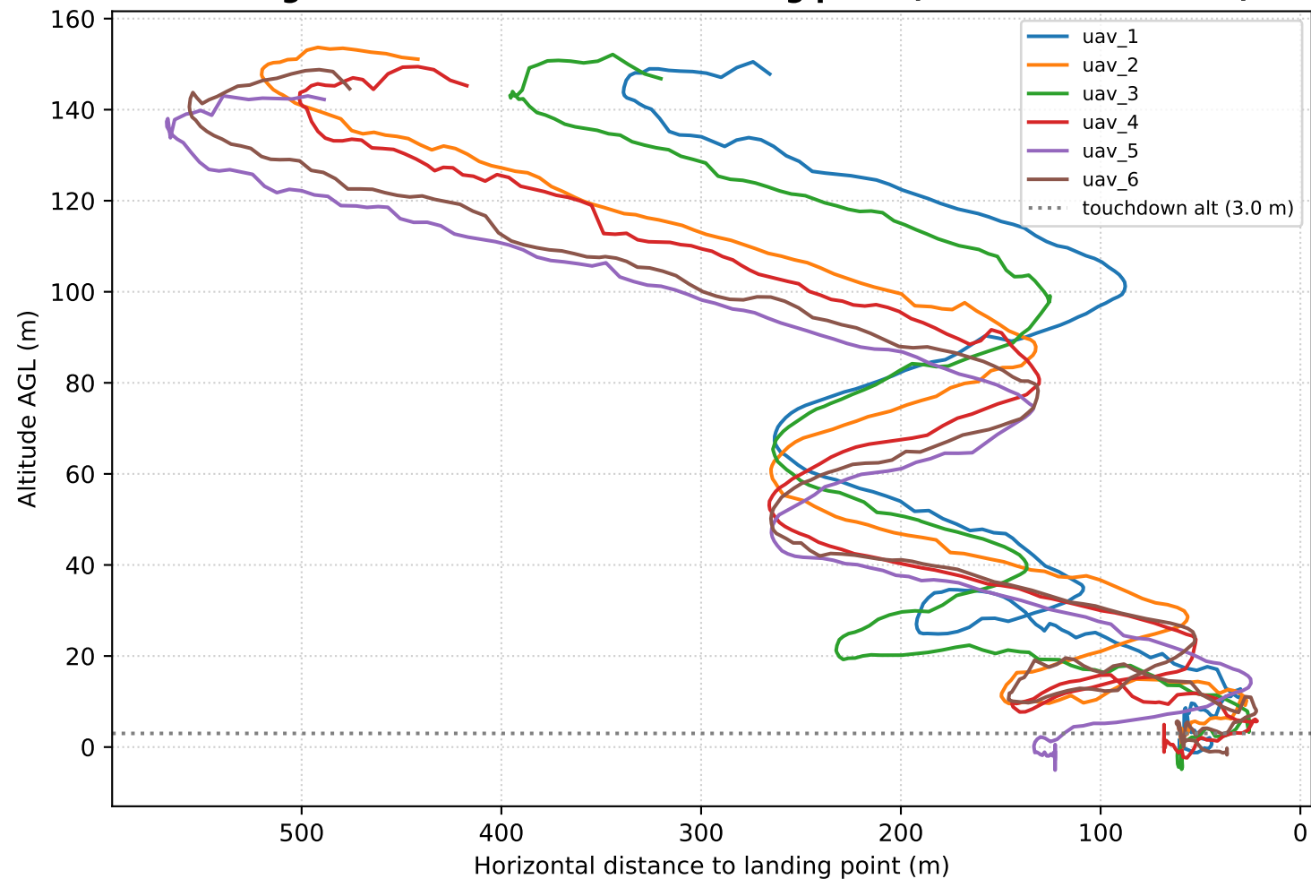
Landing altitude vs distance to landing point (continuous descent)
