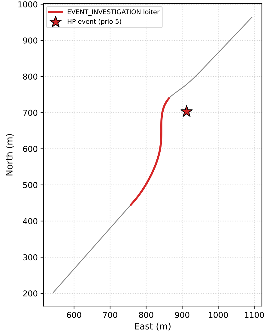
HP-event investigation (UAV 1, event 4)
