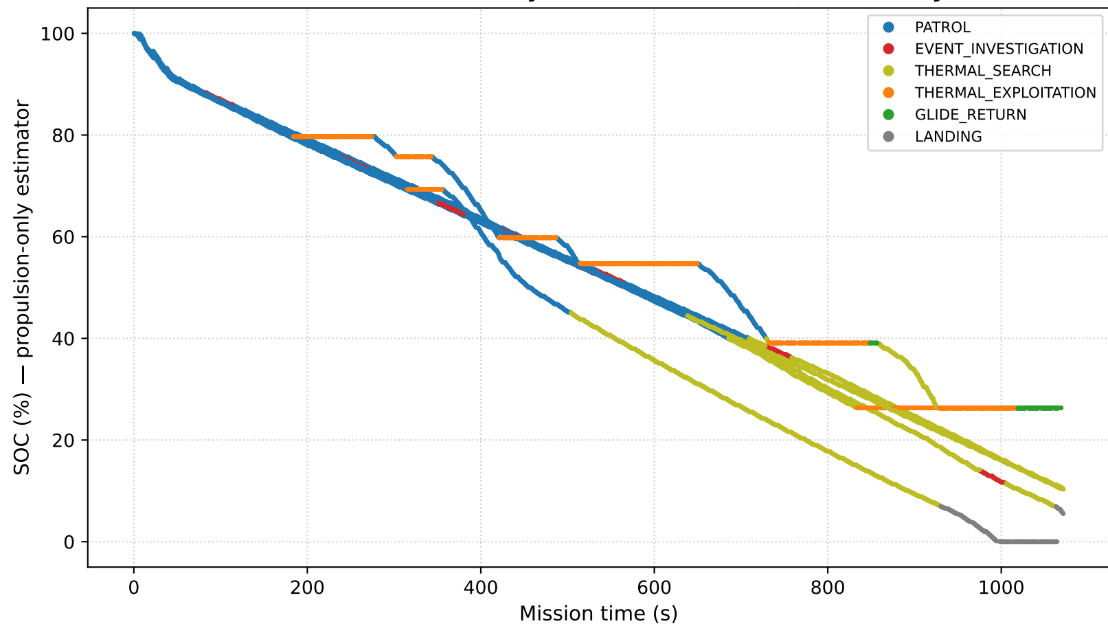
SOC time series coloured by FSM mode (all UAVs, case-study run)
