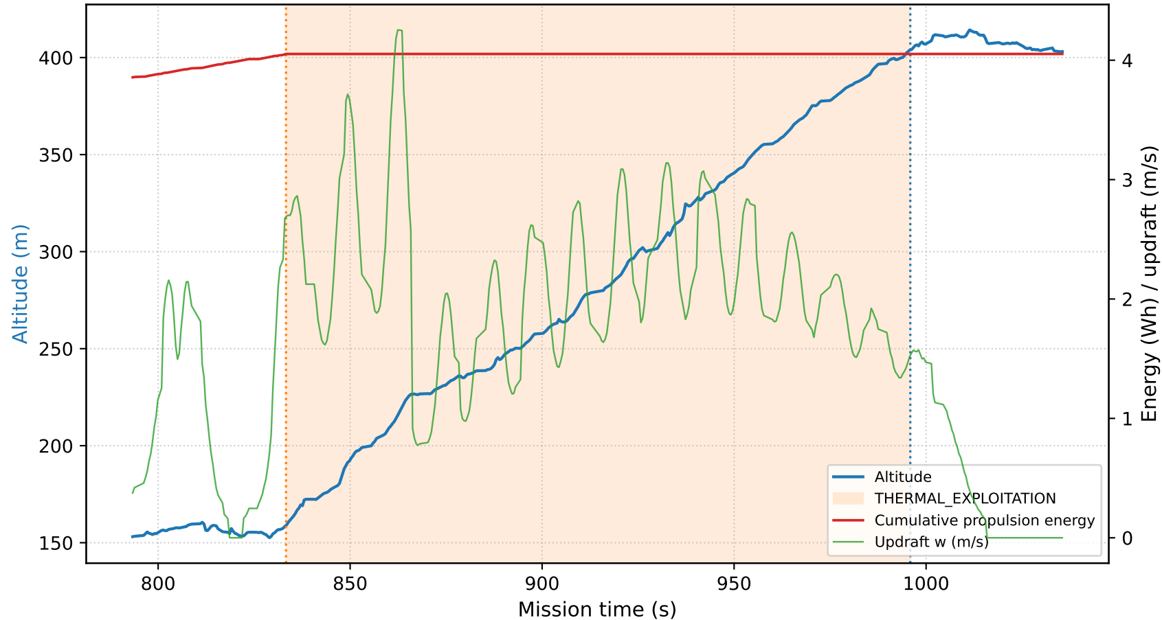
Thermal exploitation trace — UAV 3: 163 s in thermal, altitude gain +245 m, propulsion energy during segment 0.002 Wh (motor-off thermalling: energy curve is flat inside the segment)
