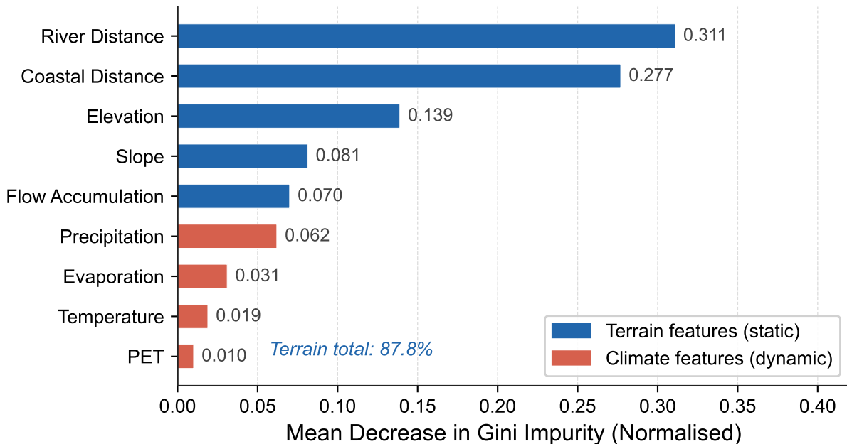
Figure 3. Random Forest Feature Importance — Indus Delta
