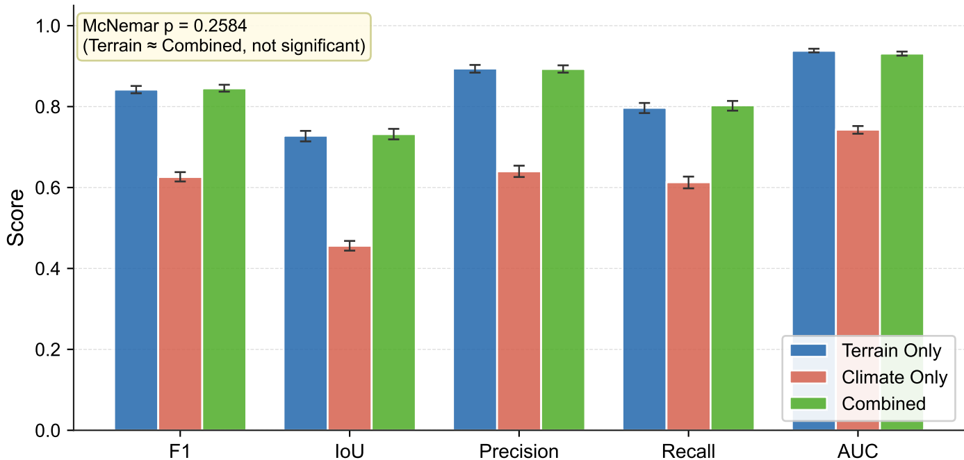
Figure 6. Feature Split Ablation — 95% Bootstrap CI, Extreme Flood Test Period
