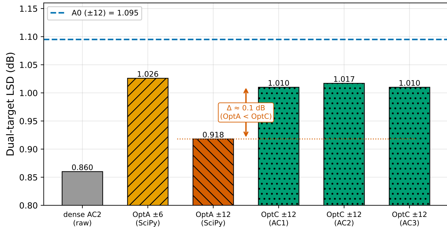
Biquad reduction ceiling (AC2_GRU): OptA(0.918) \neq OptC( \sim 1.01 ) at \pm 12 [OptD naive 7-pt sampling = 7.755 dB, off-scale]
