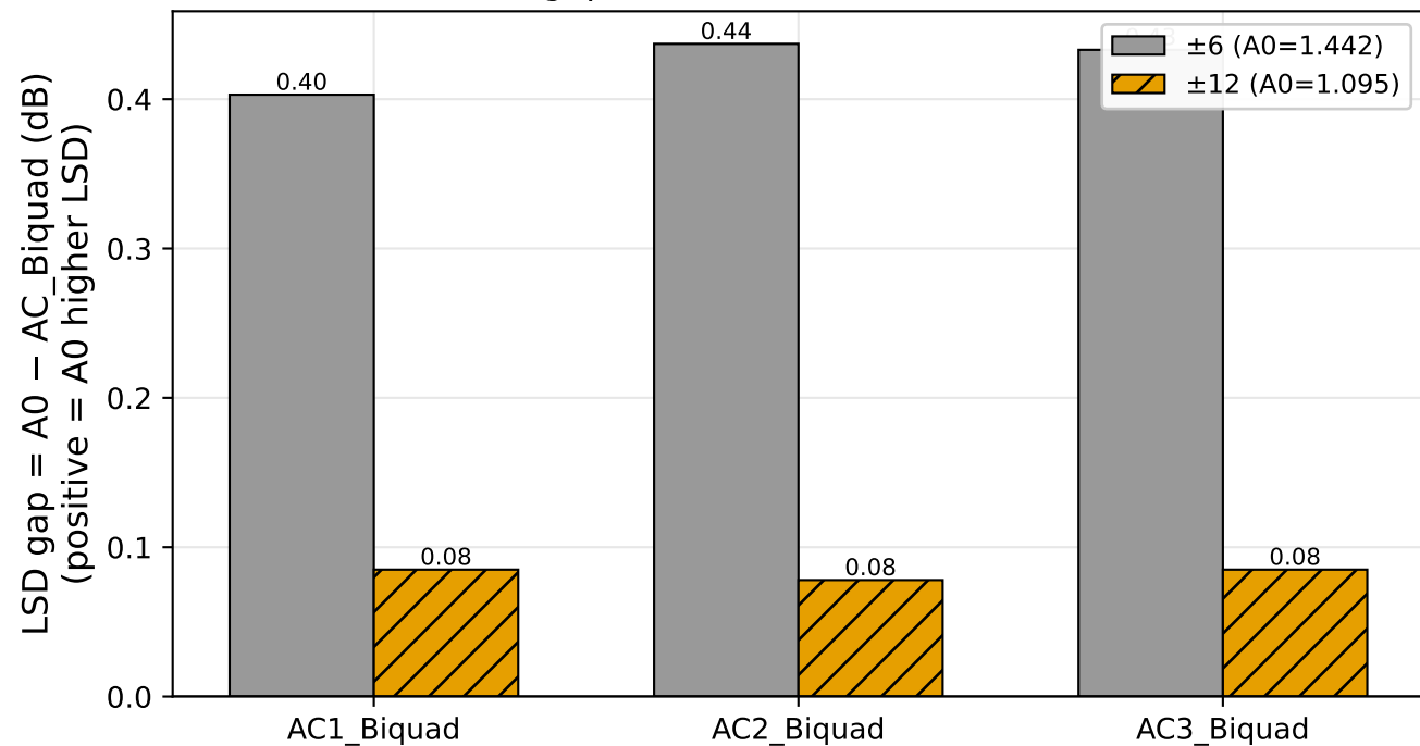
A0 vs AC_Biquad under identical 7-band \pm 12 constraint: gap shrinks \sim 0.4 \rightarrow \sim 0.08 dB
