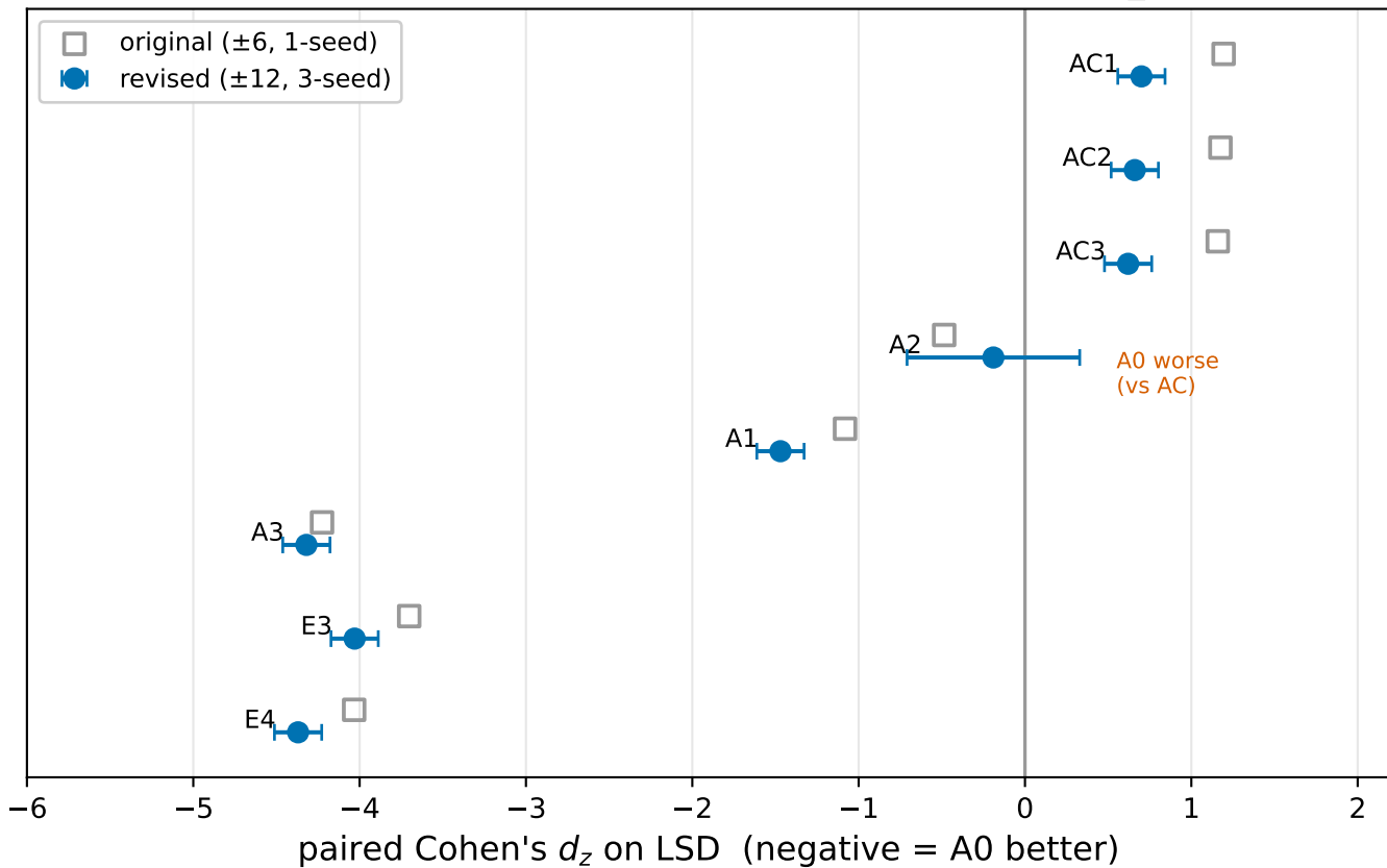
A0 vs each model — paired effect size (sample-level, test_synth)
