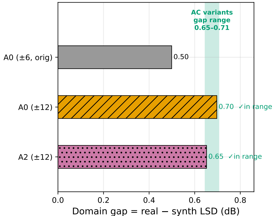
A0( \pm 12 ) gap 0.70 lies within the AC normal range (not an overfit anomaly)
