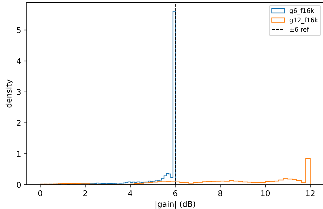
per-section |gain|
