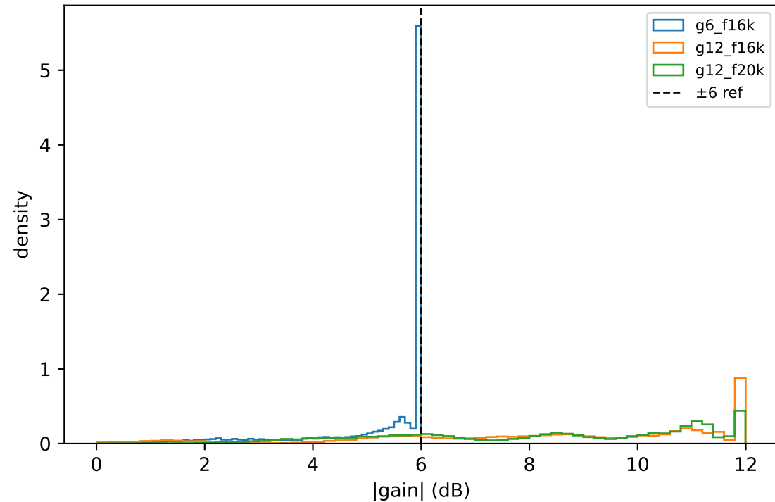
per-section |gain|
