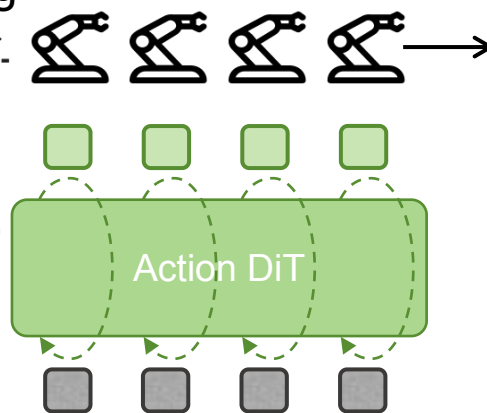
W2A (Ours): Distill world prior to action DiT
