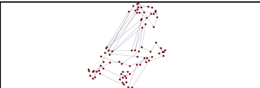
Zero-shot
