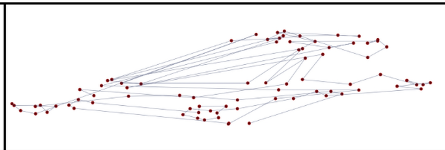
Zero-shot
