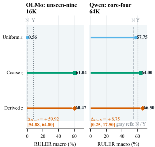
(c) Frozen pure- z zero-training
