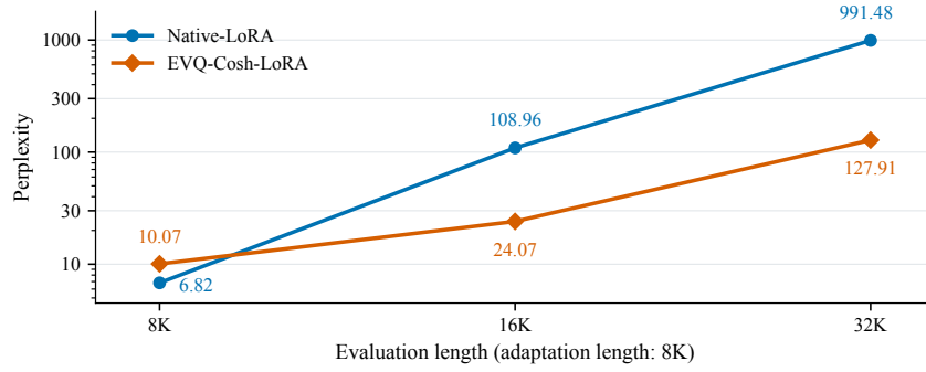
Figure 12: Cosh allocation improves extrapolation under matched adaptation. PPL is the exponential of equal-domain mean NLL.
