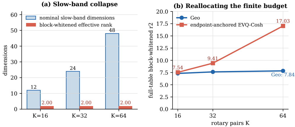
Figure 7: Spectral-budget anatomy across channel counts. Panel (a) uses the endpoint-inclusive diagnostic grid at L=4096 and b=500K : as K grows from 16 to 64, the nominal dimension assigned to pairs with \omega L \leq 1 grows from 12 to 48, while their phase-invariant effective rank remains approximately two. Panel (b) evaluates the complete fixed-endpoint table under the same uniform separation prior, using the zero-search reference \tau=2K/\sqrt{L} ; anchored EVQ-COSH spends progressively more of the available full-pair dimension than Geo as the budget grows.
