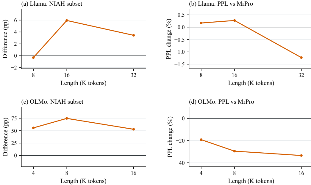
Figure 15: NIAH and language-modeling responses. NIAH is a subset of each model’s depth-balanced RULER-13 panel. Both columns show TailSpline relative to MrPro; PPL changes use each length’s absolute PPL. Llama’s 8/16K PPL slightly increases, while OLMo improves at every measured length. The panels have separate vertical scales.
