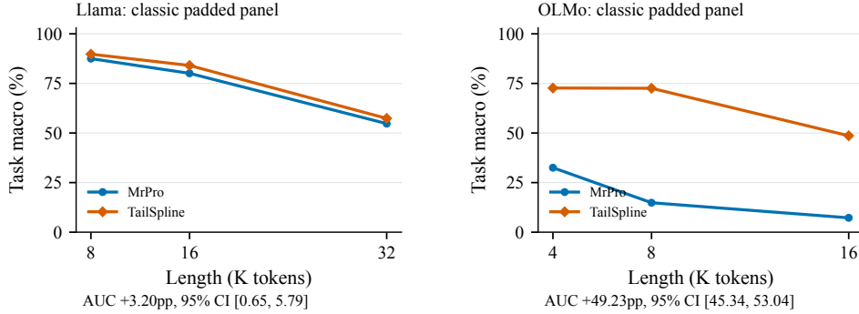
Figure 16: Classic length responses on Llama and OLMo. Each model uses its recorded depth-selected, prefix-padded input protocol. Curves and log-length AUC intervals complement the clean length panels in the main text.
