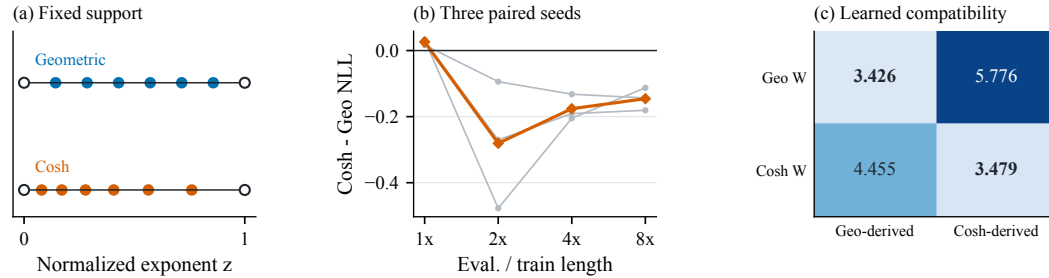
Figure 1: Fixed-support allocation and learned compatibility. (a) Fixed endpoints leave internal spacing free ( K = 8 illustration). (b) Three paired training seeds favor Cosh at extended lengths with retained support; native NLL increases. (c) Two-seed mean tail NLL for the 151.9M weights-by-derived-table crossing at 1K. Rows freeze trained weights; columns install runtime tables. The matched diagonals outperform the crossed installations.
