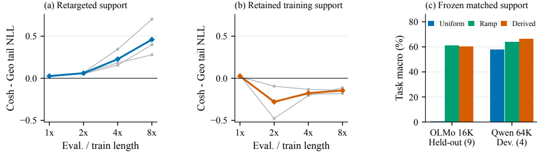
Figure 11: Allocation gains depend on the support policy. (a,b) Cosh-minus-Geo tail NLL for the same three paired 151.9M models: retargeted support ( b = L_{\text{eval}} ) versus retained training support ( b = 256 ). Thin lines show seeds; thick lines their means; 1\times = 256 tokens. Geo is the matched geometric control. (c) Frozen matched-support tasks: OLMo’s nine held-out and Qwen’s four development tasks, 20 inputs/task, with shared endpoints, amplitude, weights and inputs within each model.
