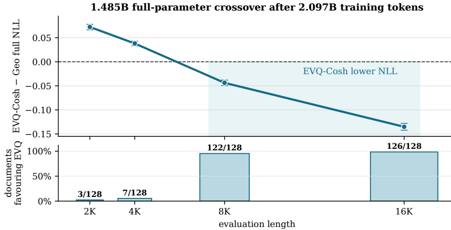
Figure 13: Full-parameter scale evidence crosses beyond the training window. The 1.485B Geo and EVQ-COSH arms start from the same public initialisation and follow the same scientific recipe for 2.097B tokens. Error bars are paired bootstrap intervals over the same 128 held-out documents, conditioned on this trained pair; the lower panel gives the document count favouring EVQ-COSH at each length.
