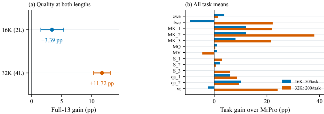
Figure 4: TailSpline improves task quality at both 2L and 4L. Clean source-order RULER with one static s = 4 table. (a) Full-13 task-equal gains and paired 95% intervals. (b) All task differences at each length; 16K uses 50 inputs per task and 32K uses 200. MK, MQ, MV and S denote multikey, multiquery, multivalue and single-key retrieval.
