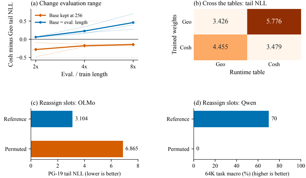
Figure 17: Three interventions distinguish the supplied spectrum from learned compatibility. (a) Range retargeting reverses the ordering of the same trained allocations; thin lines are three seeds and thick lines their means. (b) Crossed factor-four tables at 1K: rows are trained weights, columns runtime tables, and cells are mean tail NLL over two seeds and 32 anchors/seed. (c,d) Permuting interior frequency assignments preserves the final frequency multiset, endpoints and gain, but changes OLMo PG-19 tail NLL and Qwen 64K task macro (4 tasks, 20 rows/task). Each metric has its own axis. Joint Q/K compensation is the algebraic identity in (68), not a plotted recovery experiment.
