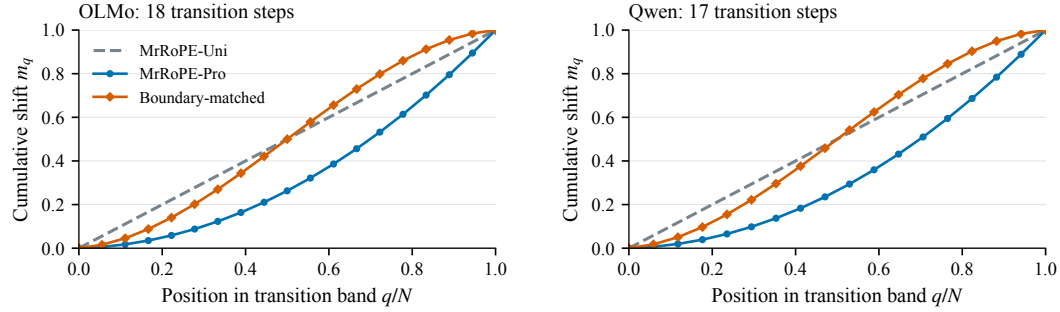
Figure 14: Intermediate-band exponent displacements. All three profiles have the same cumulative scale at the endpoints. BM redistributes the increments toward the middle of the transition band.
