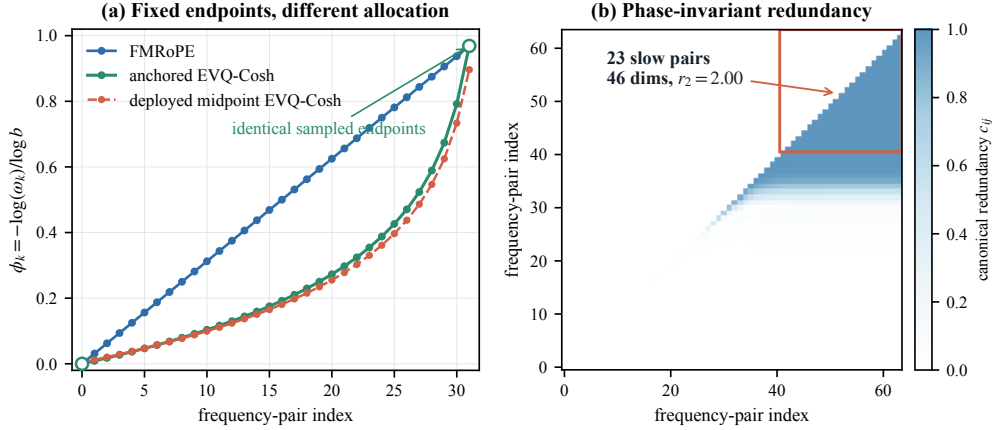
Figure 6: Where a finite frequency table spends its budget. (a) At K=32 , Cosh concentrates interior channels toward the fast end while endpoint normalisation preserves sampled support; the deployed midpoint table is shown separately. (b) For standard RoPE at L=4096 , b=5 \times 10^5 , and K=64 , phase-invariant full-subspace redundancy concentrates in the 23 pairs with \omega L \leq 1 .
