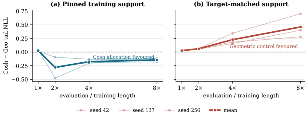
Figure 9: Support and interior allocation are distinct design coordinates. Each thin line is one training seed and the heavy line is the mean. At pinned training support, all three seeds favour anchored EVQ-COSH at every OOD length (a). Retargeting each arm’s support reverses all three OOD comparisons (b). The fixed-support panel isolates the allocation effect; the tested target-matched policy reverses the ordering of the two tested policies.
