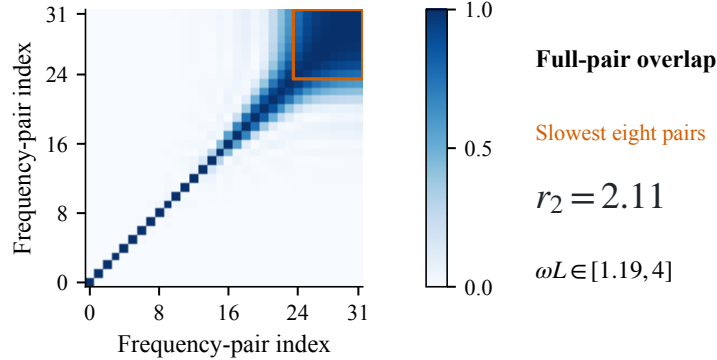
Figure 8: Slow pairs share positional directions. Full-pair canonical overlap on b = 256 , K = 32 , L = 256 under uniform separations. The slowest eight pairs have r_2 = 2.11 despite \omega L \in [1.19, 4] .
