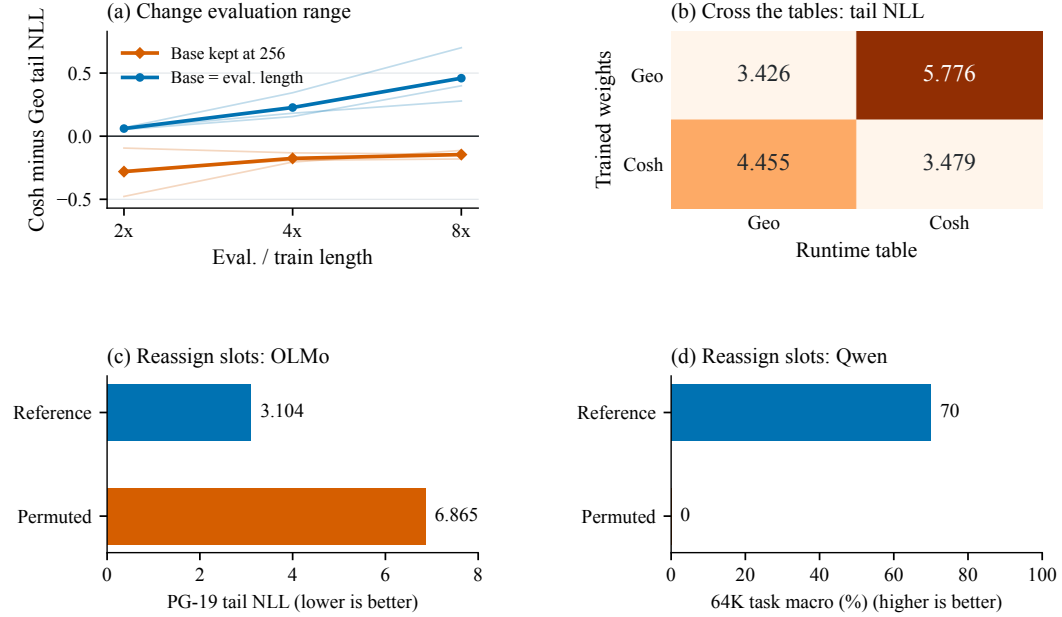
Figure 12: Three interventions distinguish the supplied spectrum from learned compatibility. (a) Range retargeting reverses the ordering of the same trained allocations; thin lines are three seeds and thick lines their means. (b) Crossed factor-four tables at 1K: rows are trained weights, columns runtime tables, and cells are mean tail NLL over two seeds and 32 anchors/seed. (c,d) Permuting interior frequency assignments preserves the final frequency multiset, endpoints and gain, but changes OLMo PG-19 tail NLL and Qwen 64K task macro (4 tasks, 20 rows/task). Each metric has its own axis. Joint Q/K compensation is the algebraic identity in (62), not a plotted recovery experiment.
