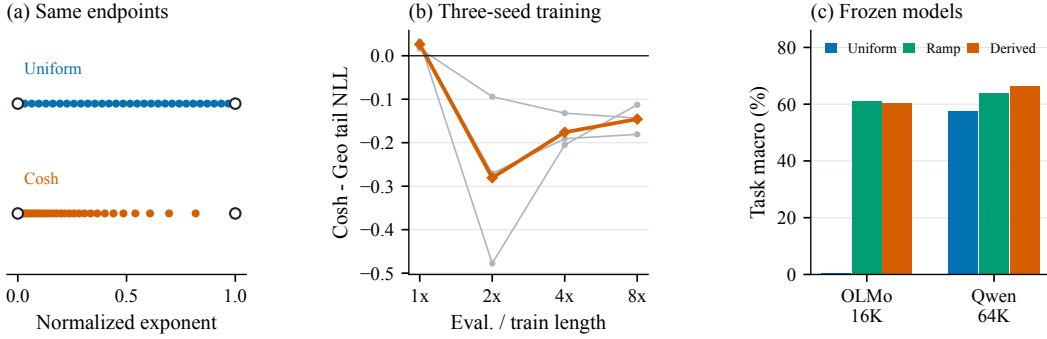
Figure 2: Internal allocation improves extrapolation and frozen-model tasks. (a) Uniform and anchored Cosh allocations share both sampled endpoints and 32 rotary pairs. (b) Cosh-minus-Geo tail NLL at the training length ( 1\times = 256 ) and three extended lengths. Thin lines are the three paired training seeds; the thick line is their mean. (c) Frozen matched-support interventions: OLMo has nine held-out tasks and Qwen four development tasks, each with 20 inputs/task. The uniform, coarse-ramp and derived arms share endpoints, amplitude, weights and inputs.
