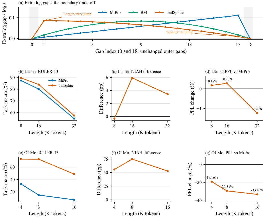
Figure 4: Explicit boundary design and training-free gains. (a) At n = 17 , TailSpline accepts a larger entry jump than MrPro to reduce the tail jump. Rows show Llama (8/16/32K) and OLMo (4/8/16K); columns show depth-balanced RULER-13 macro, its NIAH subset difference, and relative PPL change versus MrPro. PPL axes have different scales; absolute PPL is in Appendix H. Arms share band, endpoints, gain and inputs within each model.
