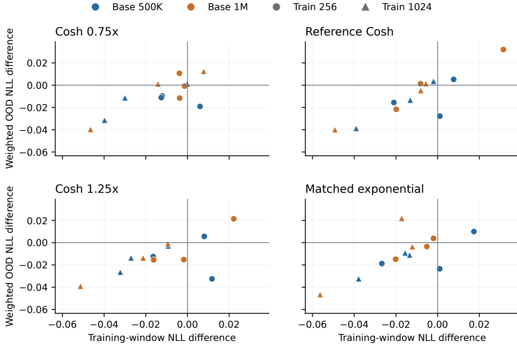
Figure 8: Allocation changes training-window and extended-length loss jointly. Each point is one of the twelve prespecified M4 configurations, averaging three paired seeds; all four nonuniform main arms are shown. Both axes are differences from the matching geometric arm, so negative values improve loss. OOD weights are proportional to \log_2(r + 1) for r \in \{2, 4, 8\} , as in the original protocol. The horizontal coordinate is reconstructed from recorded four-decimal PPL; the vertical coordinate uses the recorded full-precision weighted NLL. The configurations form a prespecified design grid.
