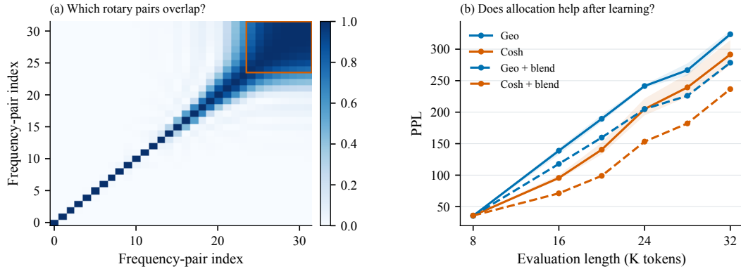
Figure 3: Finite-window geometry and learning-time allocation. (a) Full-pair canonical overlap on the b = 256 , K = 32 , L = 256 identification grid under uniform separation measure. (b) Three-seed mean PPL of the 432M MLA extrapolation evaluation. Solid curves use trained tables; dashed curves apply the same wavelength blend ( s = 4 ). Shading is the three-seed range.
