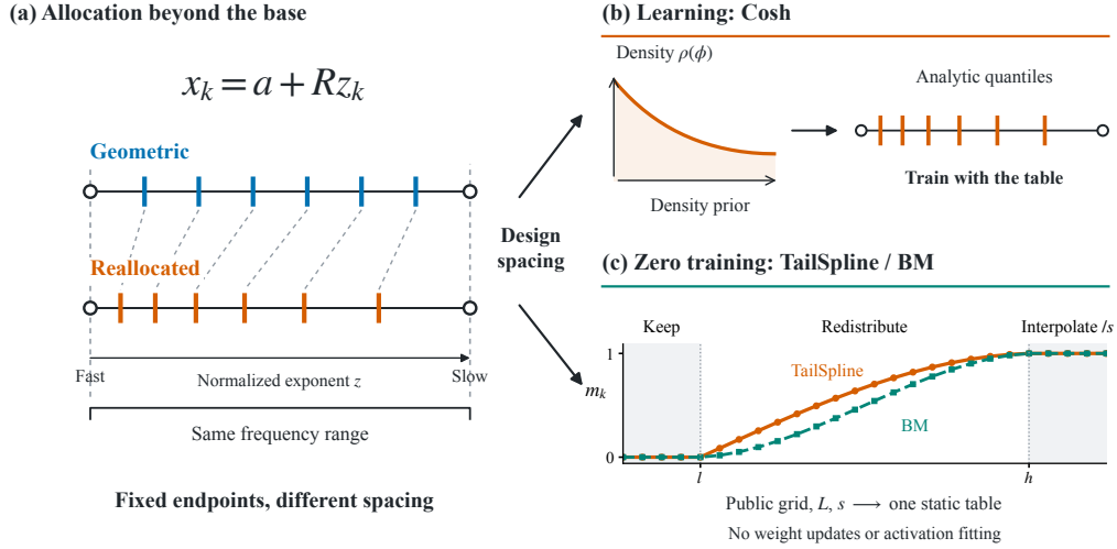
Figure 1: Allocation is a design freedom with learning and zero-training uses. (a) Fixed endpoints leave internal spacing free. (b) Cosh turns a density prior into a finite table through quantiles. These illustrations use K = 8 , \tau = 2 and endpoint anchoring. (c) Exact TailSpline and BM profiles at n = 17 redistribute extension between unchanged high frequencies and a tail scaled by 1/s . The two routes use distinct objectives to design frequency spacing.
