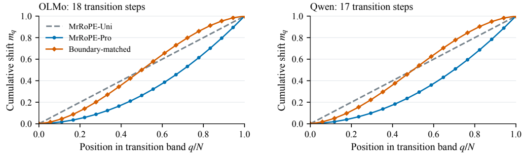
Figure 11: Intermediate-band exponent displacements. All three profiles have the same cumulative scale at the endpoints. BM redistributes the increments toward the middle of the transition band.
