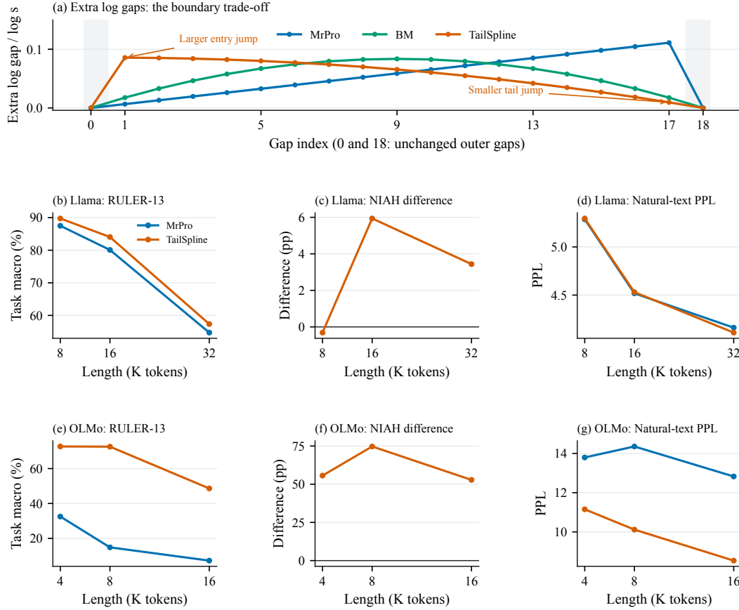
Figure 3: Explicit boundary design and training-free gains on two model families. (a) At n = 17 , TailSpline accepts a larger entry jump than MrPro to reduce the tail jump; outer extra gaps are zero. Rows show Llama (8/16/32K) and OLMo (4/8/16K); columns show RULER-13 macro, NIAH paired difference, and PPL. Within each model, arms share band, endpoints, gain and inputs. NIAH is a RULER subset. Lines join measured points.
