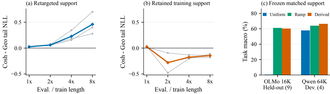
Figure 2: Allocation gains depend on the support policy. (a,b) Cosh-minus-Geo tail NLL for the same three paired 151.9M models: retargeted support ( b = L_{\text{eval}} ) versus retained training support ( b = 256 ). Thin lines show seeds; thick lines their means; 1\times = 256 tokens. Geo is the matched geometric control. (c) Frozen matched-support tasks: OLMo’s nine held-out and Qwen’s four development tasks, 20 inputs/task, with shared endpoints, amplitude, weights and inputs within each model.
