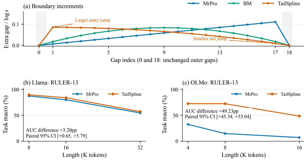
Figure 5: TailSpline improves over MrPro on the matched panels. (a) At n = 17 , TailSpline trades a larger entry jump for a smaller tail jump. (b,c) Depth-balanced RULER-13 curves; annotations give log-length AUC differences and paired 95% intervals, not per-length intervals. Arms share band, endpoints, gain and inputs within each model. NIAH/PPL responses are in Appendix H.
