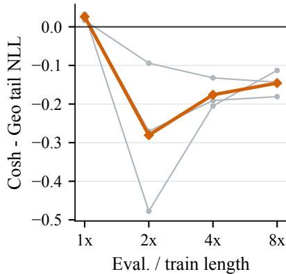
(b) Three-seed training
