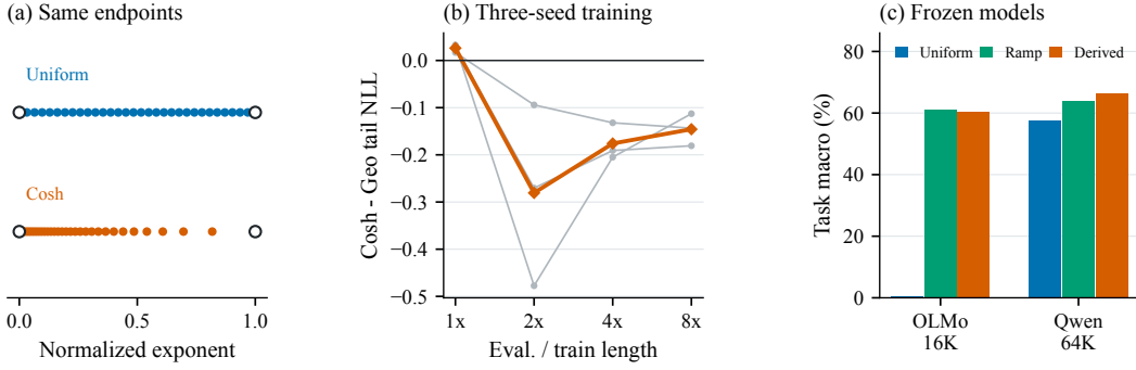
Figure 2: Internal allocation improves extrapolation and frozen-model tasks. (a) Uniform and anchored Cosh allocations share both sampled endpoints and 32 rotary pairs. (b) Cosh-minus-Geo tail NLL at the training length ( 1\times = 256 ) and three extended lengths. Thin lines are the three paired training seeds; the thick line is their mean. (c) Frozen matched-support interventions: OLMo has nine held-out tasks and Qwen four development tasks, each with 20 inputs/task. The uniform, coarse-ramp and derived arms share endpoints, amplitude, weights and inputs. Training-window costs remain visible in (b).
