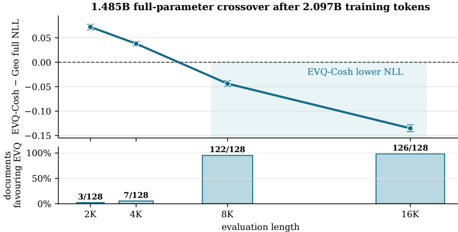
Figure 10: Full-parameter scale evidence crosses beyond the training window. The 1.485B Geo and EVQ-COSH arms start from the same public initialisation and follow the same scientific recipe for 2.097B tokens. Error bars are paired bootstrap intervals over the same 128 held-out documents, conditioned on this trained pair; the lower panel gives the document count favouring EVQ-COSH at each length.
