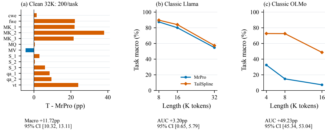
Figure 4: TailSpline improves frozen long-context performance. (a) Source-order RULER-200 at 32K: T-P differences across all tasks, with task-equal aggregate and paired 95% interval. (b,c) Llama and OLMo length responses under the classic depth-selected, prefix-padded protocol, with log-length AUC intervals.
