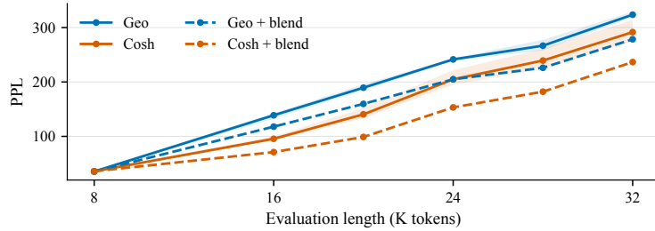
Figure 3: Cosh improves extrapolation across training seeds. Three-seed mean and range for the 432M MLA model; dashed curves use the common wavelength blend ( s = 4 ). Evaluation uses common text chunks across arms (Appendix E.1).
