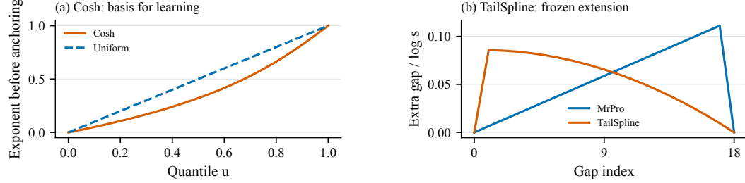
Figure 2: One design variable, two operating settings. (a) Cosh allocates the positional basis for learning, shown as quantiles before endpoint anchoring ( \tau = 2 ). (b) TailSpline allocates extra log-frequency span around a native table, smoothing the connection to the extended low-frequency tail ( n = 17 ).
