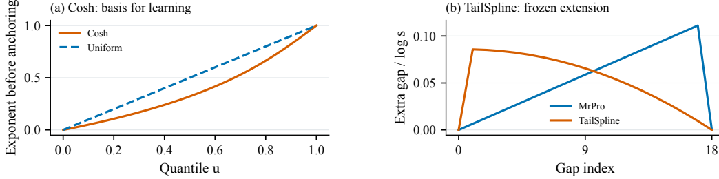
Figure 2: Explicit ways to change allocation. (a) Cosh transports frequencies for extrapolation, shown as quantiles before endpoint anchoring ( \tau = 2 ). (b) TailSpline allocates extra log-frequency span around a native table, smoothing the connection to the extended low-frequency tail ( n = 17 ).
