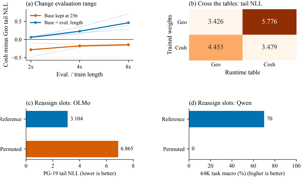
Figure 15: Three interventions distinguish the supplied spectrum from learned compatibility.
