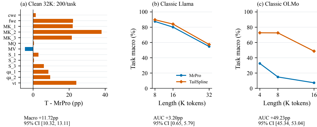
Figure 3: TailSpline improves frozen long-context performance. (a) Source-order RULER-200 at 32K: T-P differences across all tasks, with task-equal aggregate and paired 95% interval. (b,c) Llama and OLMo length responses under the classic depth-selected, prefix-padded protocol, with log-length AUC intervals.
