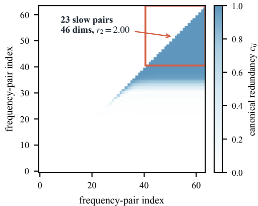
(b) Phase-invariant subspace redundancy
