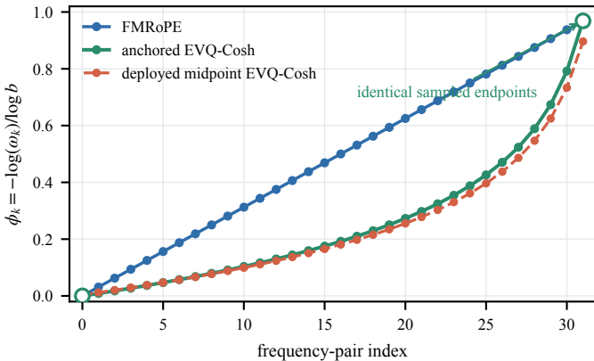
(a) The allocation axis is not the range axis
