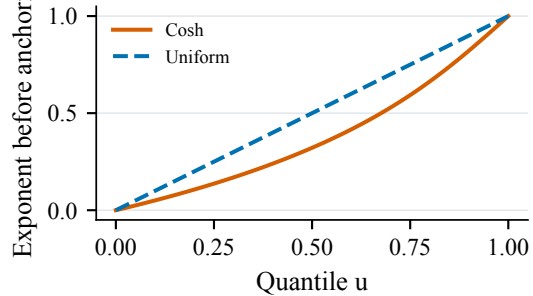
(b) Cosh: extrapolation transport
