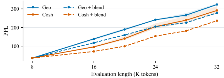
Figure 3: Cosh learning-time extrapolation. Three-seed mean PPL of the 432M MLA model; shading shows the seed range. Dashed curves use a common wavelength blend ( s = 4 ).
