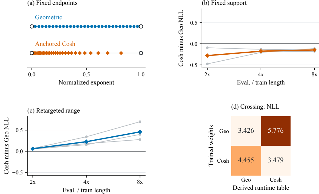
Figure 1: Interior allocation shapes learning and its use at longer ranges. (a) Two allocations share both sampled endpoints and 32 rotary pairs. (b,c) Cosh-minus-Geo tail NLL at 2 \times / 4 \times / 8 \times the 256-token training window; thin lines are three training seeds, thick lines their means. The ordering reverses when the runtime range is retargeted. (d) Crossing factor-four tables derived from the training allocations at 1K: each frozen weight set favors its corresponding table (two seeds, 32 anchors per seed).
