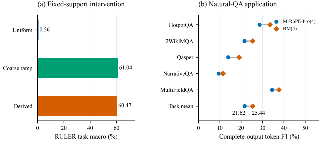
Figure 3: From a controlled allocation effect to natural-question-answering gains. (a) Frozen OLMo 16K RULER on nine held-out tasks, 20 rows/task; sampled endpoints, amplitude, weights and inputs are shared. (b) A separate matched s = 4 BM/MrRoPE-Pro comparison on five Long-Bench tasks: complete-output token F1 on 631 untruncated inputs longer than 4K. Each panel answers a different question: allocation’s effect at fixed support, and the usefulness of a concrete redistribution.
