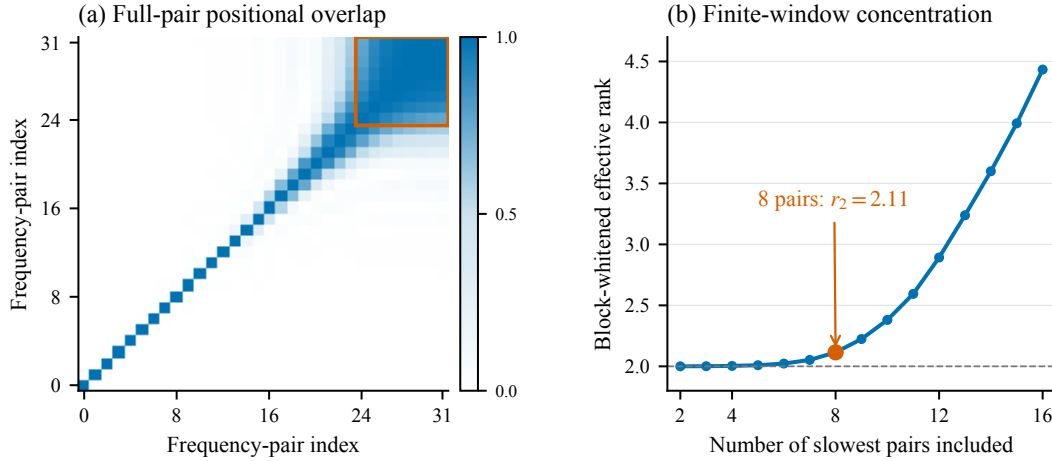
Figure 2: Log-frequency spacing and positional directions are different objects. Uniform separation measure on [0, L] . (a) Canonical overlap of full sine-cosine pairs on the actual b = 256 , K = 32 , L = 256 identification grid. The eight slowest pairs share most of their positional space. (b) Effective rank as progressively faster pairs enter that slow subset: eight pairs give 16 coordinates but r_2 = 2.11 . Values are closed-form Gram calculations checked by independent quadrature.
