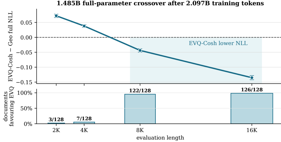
Figure 9: Full-parameter scale evidence crosses beyond the training window. The 1.485B Geo and EVQ-COSH arms start from the same public initialisation and follow the same scientific recipe for 2.097B tokens. Error bars are paired bootstrap intervals over the same 128 held-out documents, conditioned on this trained pair; the lower panel gives the document count favouring EVQ-COSH at each length.
