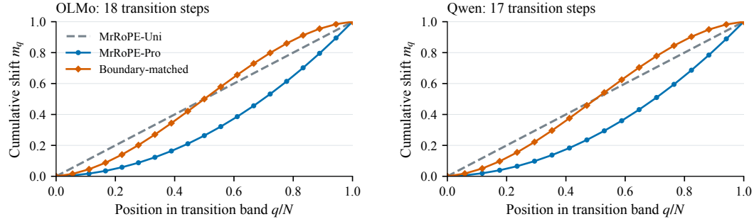
Figure 10: Intermediate-band exponent displacements. All three profiles have the same cumulative scale at the endpoints. BM redistributes the increments toward the middle of the transition band.
