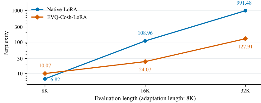
Figure 7: Cosh allocation improves extrapolation under matched adaptation . PPL is the exponential of equal-domain mean NLL.
