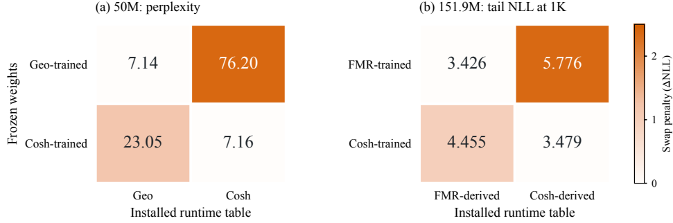
Figure 8: Weights co-adapt to their exponent allocation. Each row freezes one trained weight set and changes only its runtime table. Left: 50M crossing, PPL on eight windows. Right: 151.9M crossing, mean tail NLL on 32 anchors in each of two training seeds, using extensions derived from the two training tables. FMR is the geometric table at the fixed training range; shading shows the NLL increase relative to the matched diagonal cell.
